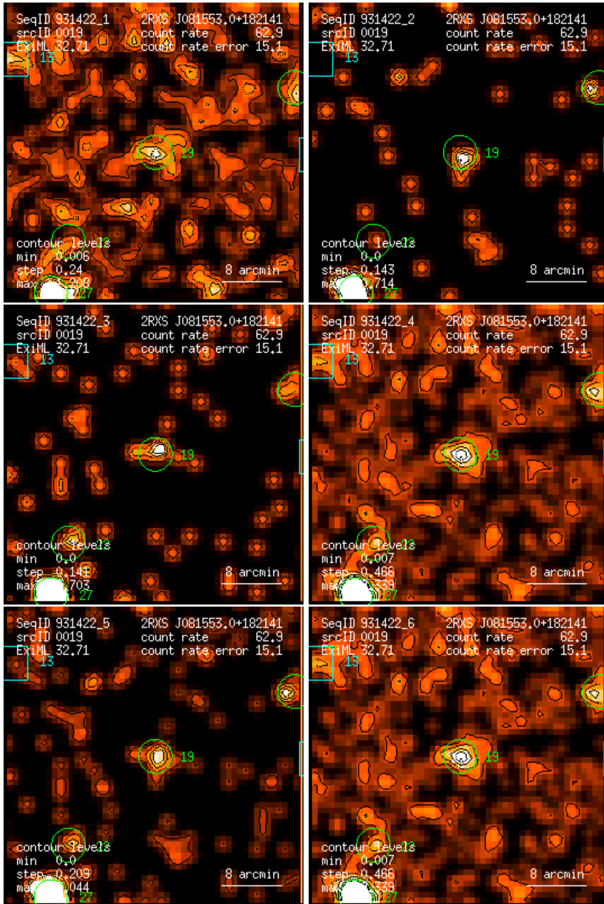
Figure 19: RASS 931422: detection 0019: band rate images, Gaussian filter: (1) PSPC channels 11 – 41, (2) 52 – 90, (3) 91 – 201, (4) 11 – 235, (5) 52 – 201, (6) 11 – 201. Broad band rates in counts/ks. Band rate contour levels in counts/ks/arcmin 2 .
