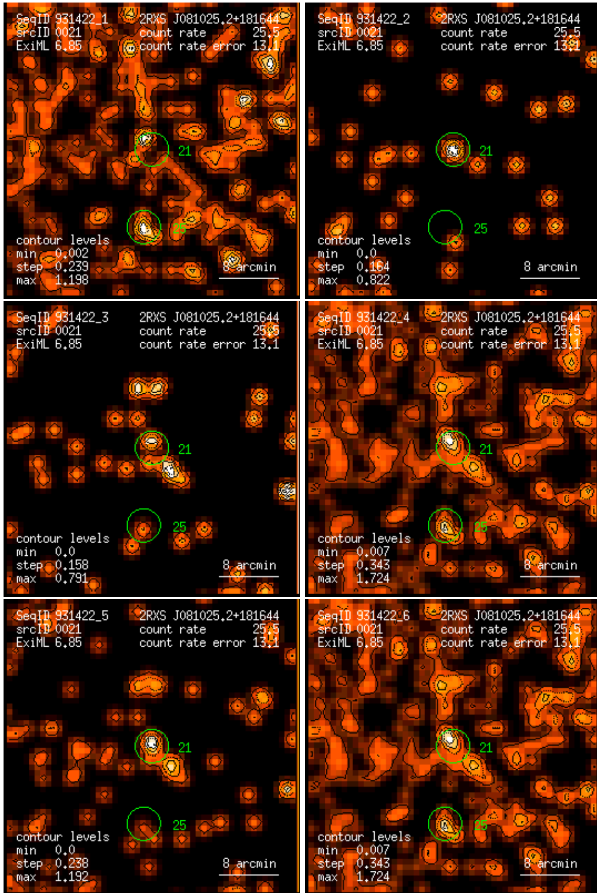
Figure 21: RASS 931422: detection 0021: band rate images, Gaussian filter: (1) PSPC channels 11 – 41, (2) 52 – 90, (3) 91 – 201, (4) 11 – 235, (5) 52 – 201, (6) 11 – 201. Broad band rates in counts/ks. Band rate contour levels in counts/ks/arcmin 2 .
