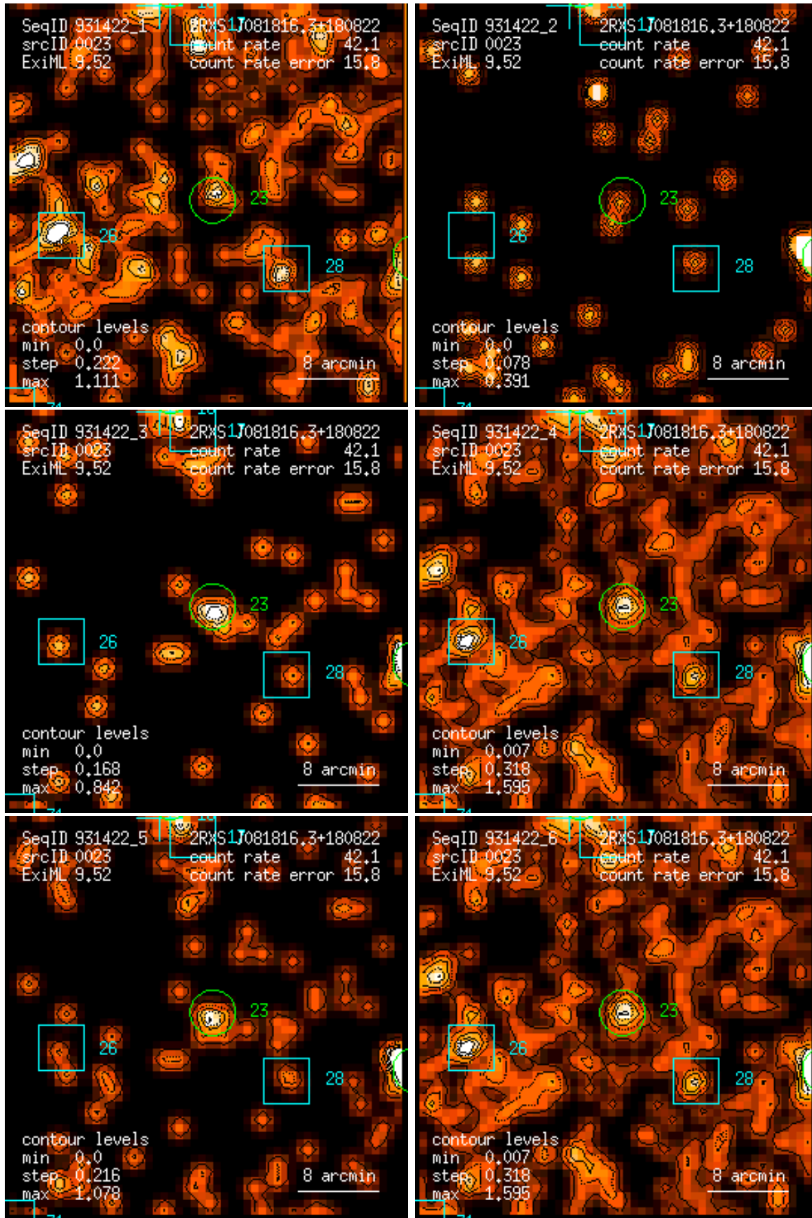
Figure 23: RASS 931422: detection 0023: band rate images, Gaussian filter: (1) PSPC channels 11 – 41, (2) 52 – 90, (3) 91 – 201, (4) 11 – 235, (5) 52 – 201, (6) 11 – 201. Broad band rates in counts/ks. Band rate contour levels in counts/ks/arcmin 2 .
