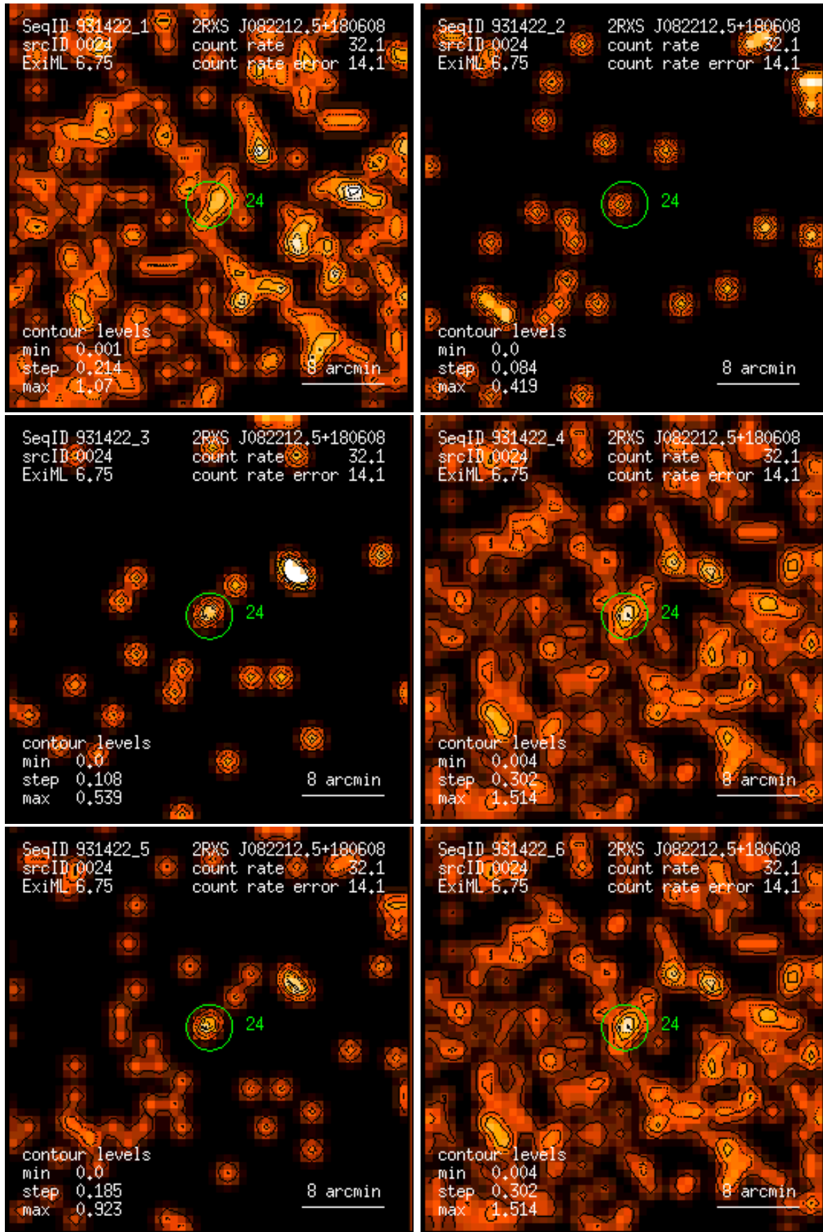
Figure 24: RASS 931422: detection 0024: band rate images, Gaussian filter: (1) PSPC channels 11 – 41, (2) 52 – 90, (3) 91 – 201, (4) 11 – 235, (5) 52 – 201, (6) 11 – 201. Broad band rates in counts/ks. Band rate contour levels in counts/ks/arcmin 2 .
