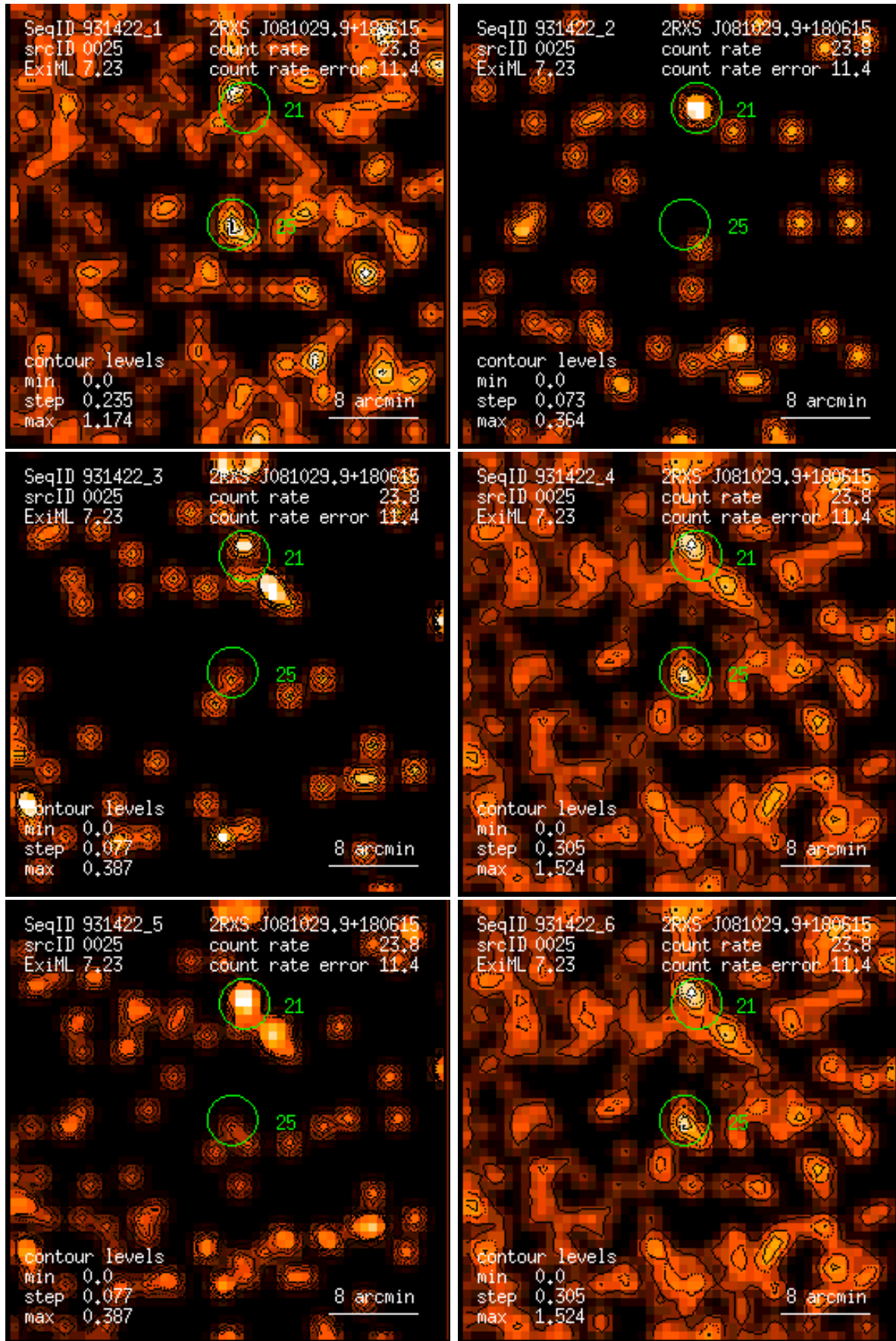
Figure 25: RASS 931422: detection 0025: band rate images, Gaussian filter: (1) PSPC channels 11 – 41, (2) 52 – 90, (3) 91 – 201, (4) 11 – 235, (5) 52 – 201, (6) 11 – 201. Broad band rates in counts/ks. Band rate contour levels in counts/ks/arcmin 2 .
