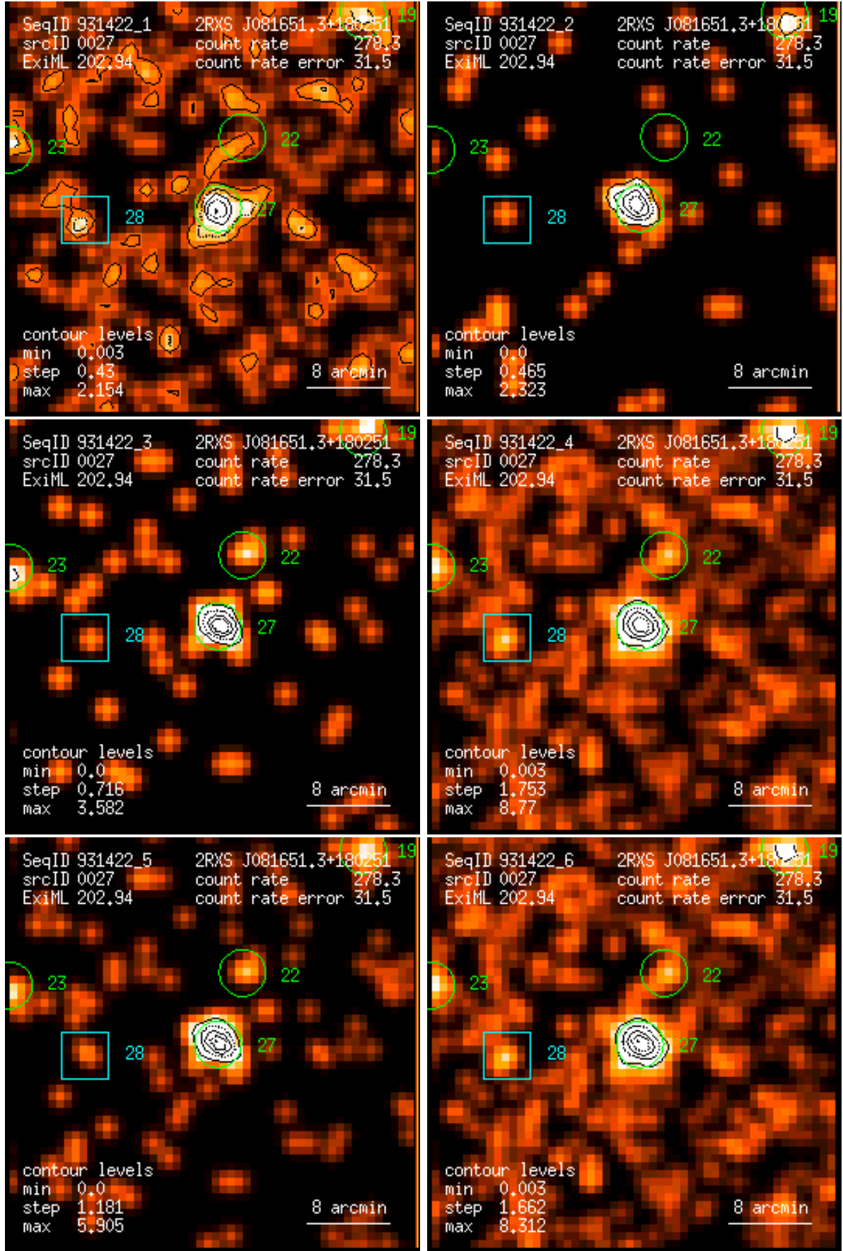
Figure 27: RASS 931422: detection 0027: band rate images, Gaussian filter: (1) PSPC channels 11 – 41, (2) 52 – 90, (3) 91 – 201, (4) 11 – 235, (5) 52 – 201, (6) 11 – 201. Broad band rates in counts/ks. Band rate contour levels in counts/ks/arcmin 2 .
