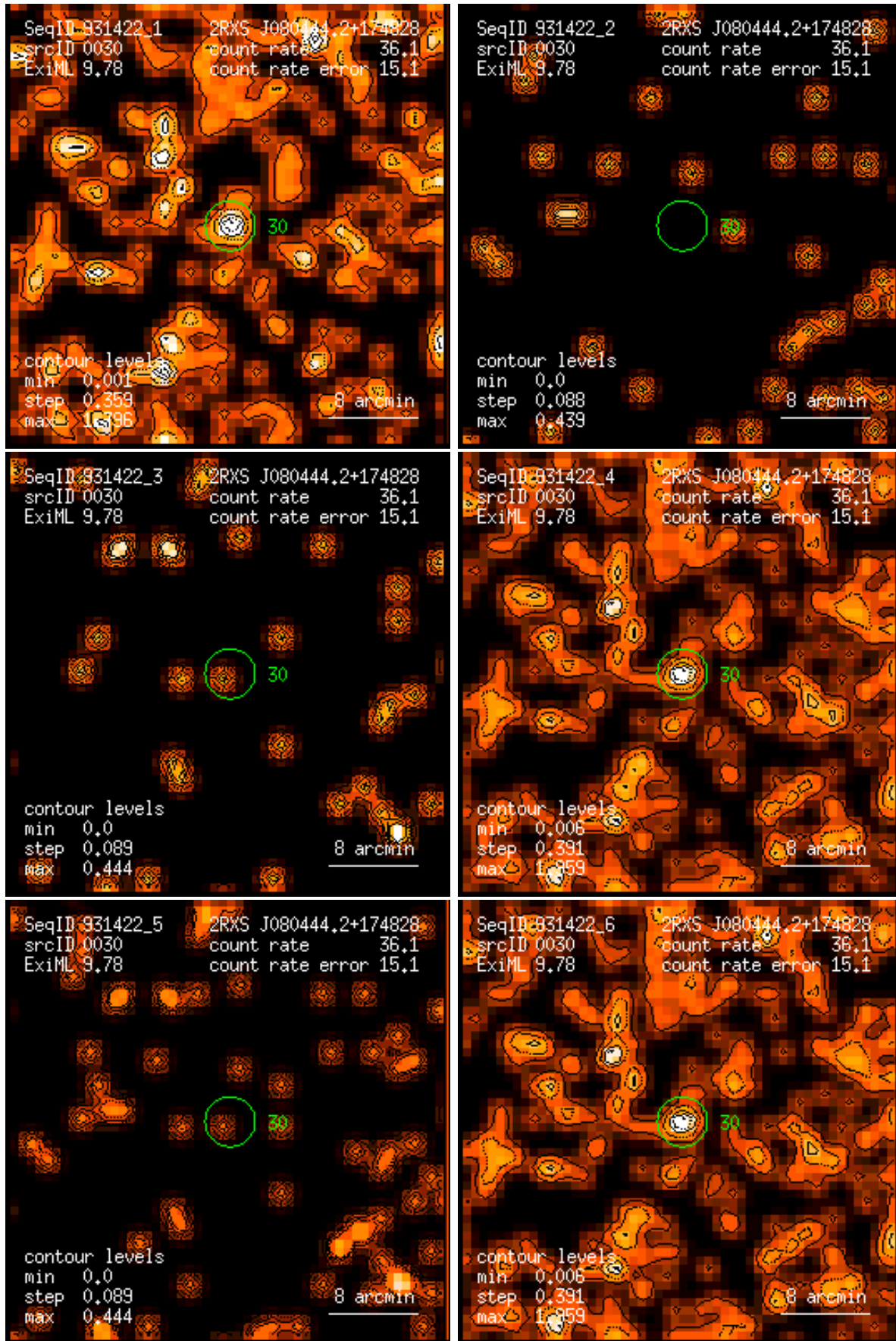
Figure 30: RASS 931422: detection 0030: band rate images, Gaussian filter: (1) PSPC channels 11 – 41, (2) 52 – 90, (3) 91 – 201, (4) 11 – 235, (5) 52 – 201, (6) 11 – 201. Broad band rates in counts/ks. Band rate contour levels in counts/ks/arcmin 2 .
