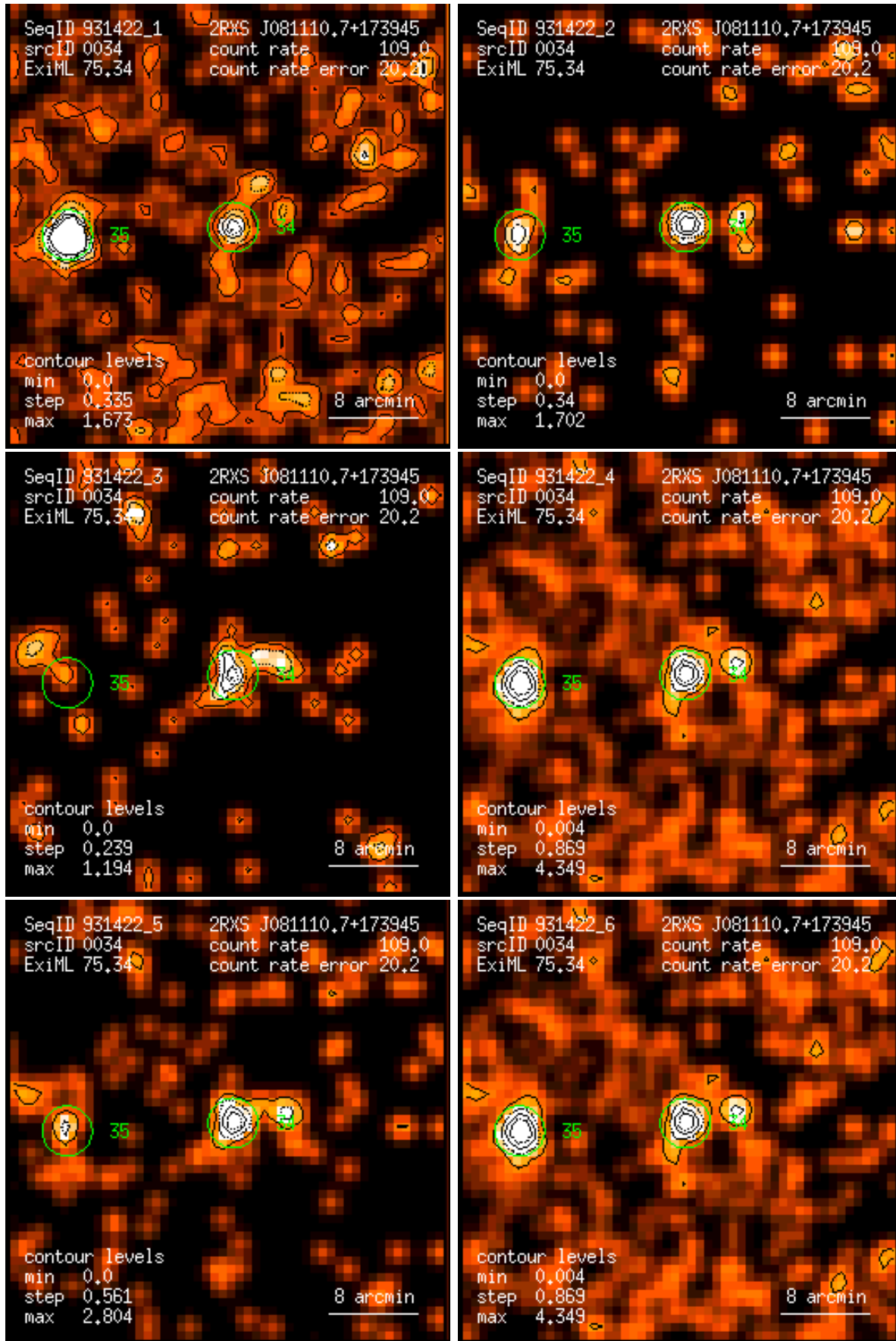
Figure 34: RASS 931422: detection 0034: band rate images, Gaussian filter: (1) PSPC channels 11 – 41, (2) 52 – 90, (3) 91 – 201, (4) 11 – 235, (5) 52 – 201, (6) 11 – 201. Broad band rates in counts/ks. Band rate contour levels in counts/ks/arcmin 2 .
