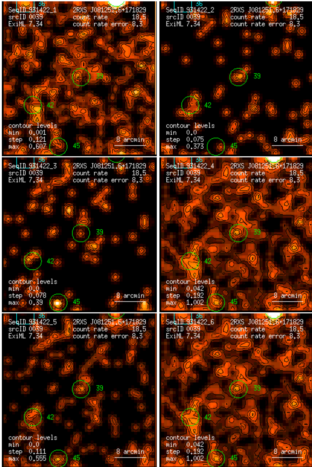
Figure 39: RASS 931422: detection 0039: band rate images, Gaussian filter: (1) PSPC channels 11 – 41, (2) 52 – 90, (3) 91 – 201, (4) 11 – 235, (5) 52 – 201, (6) 11 – 201. Broad band rates in counts/ks. Band rate contour levels in counts/ks/arcmin 2 .
