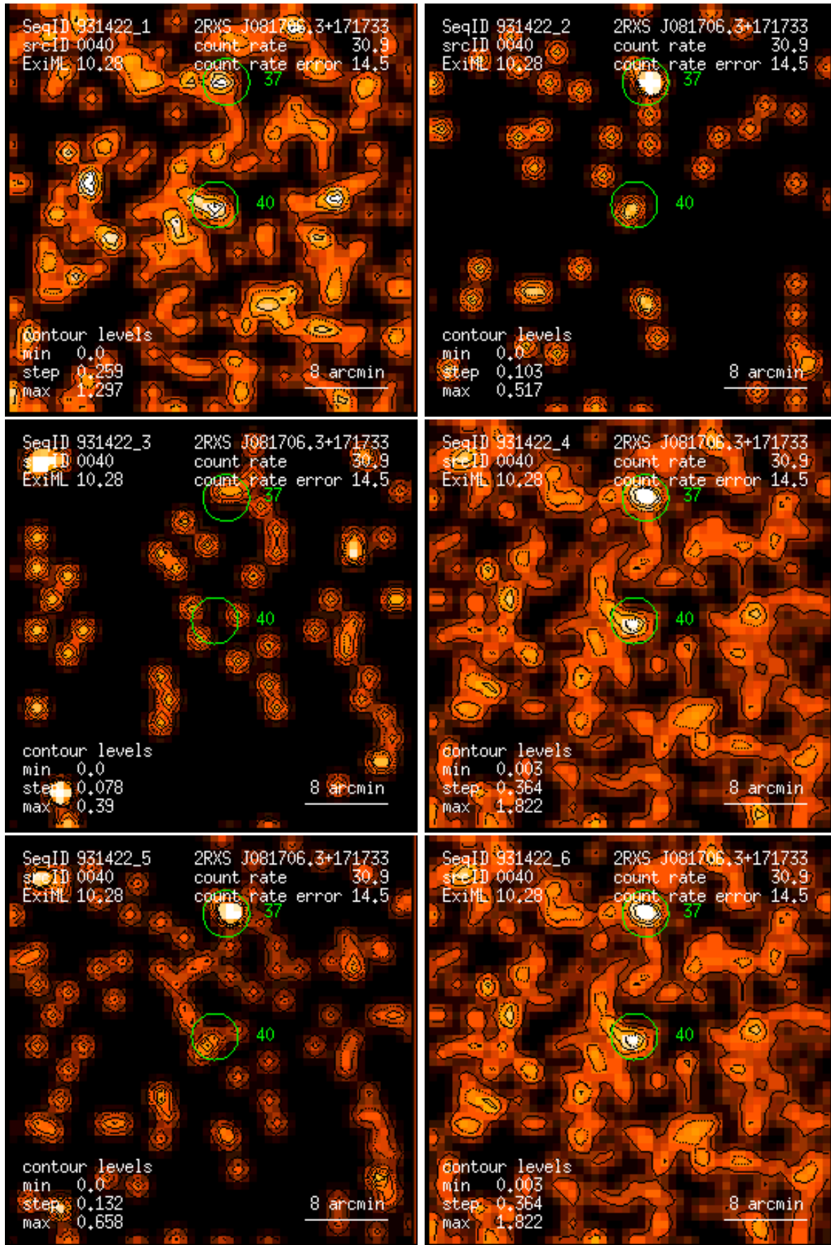
Figure 40: RASS 931422: detection 0040: band rate images, Gaussian filter: (1) PSPC channels 11 – 41, (2) 52 – 90, (3) 91 – 201, (4) 11 – 235, (5) 52 – 201, (6) 11 – 201. Broad band rates in counts/ks. Band rate contour levels in counts/ks/arcmin 2 .
