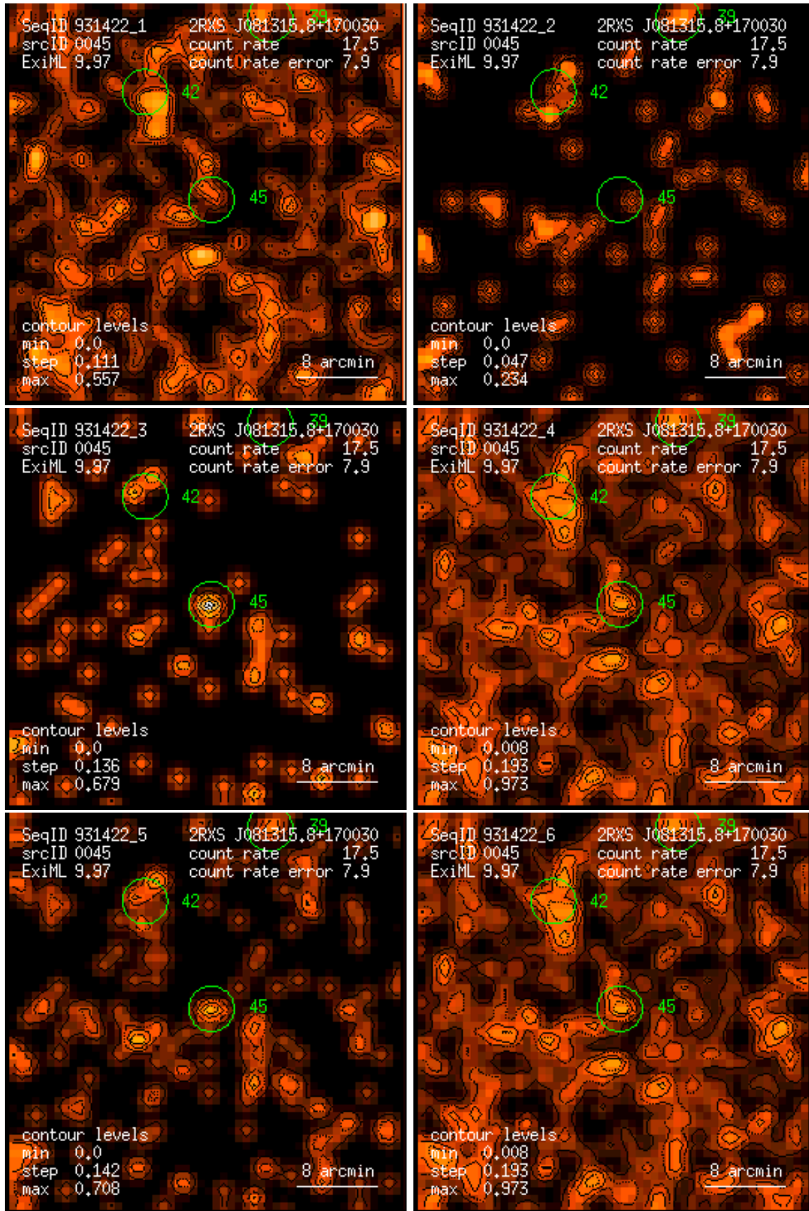
Figure 45: RASS 931422: detection 0045: band rate images, Gaussian filter: (1) PSPC channels 11 – 41, (2) 52 – 90, (3) 91 – 201, (4) 11 – 235, (5) 52 – 201, (6) 11 – 201. Broad band rates in counts/ks. Band rate contour levels in counts/ks/arcmin 2 .
