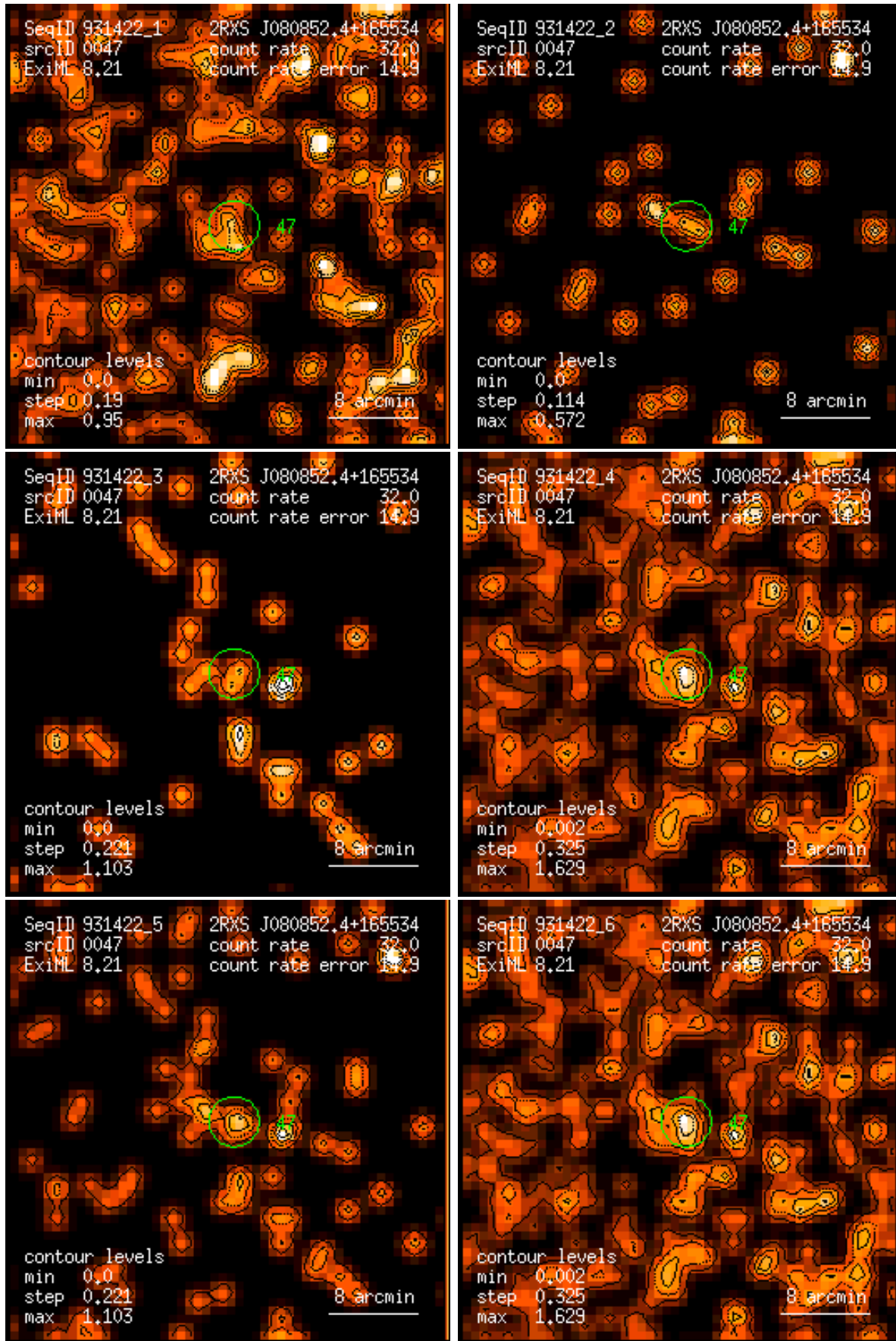
Figure 47: RASS 931422: detection 0047: band rate images, Gaussian filter: (1) PSPC channels 11 – 41, (2) 52 – 90, (3) 91 – 201, (4) 11 – 235, (5) 52 – 201, (6) 11 – 201. Broad band rates in counts/ks. Band rate contour levels in counts/ks/arcmin 2 .
