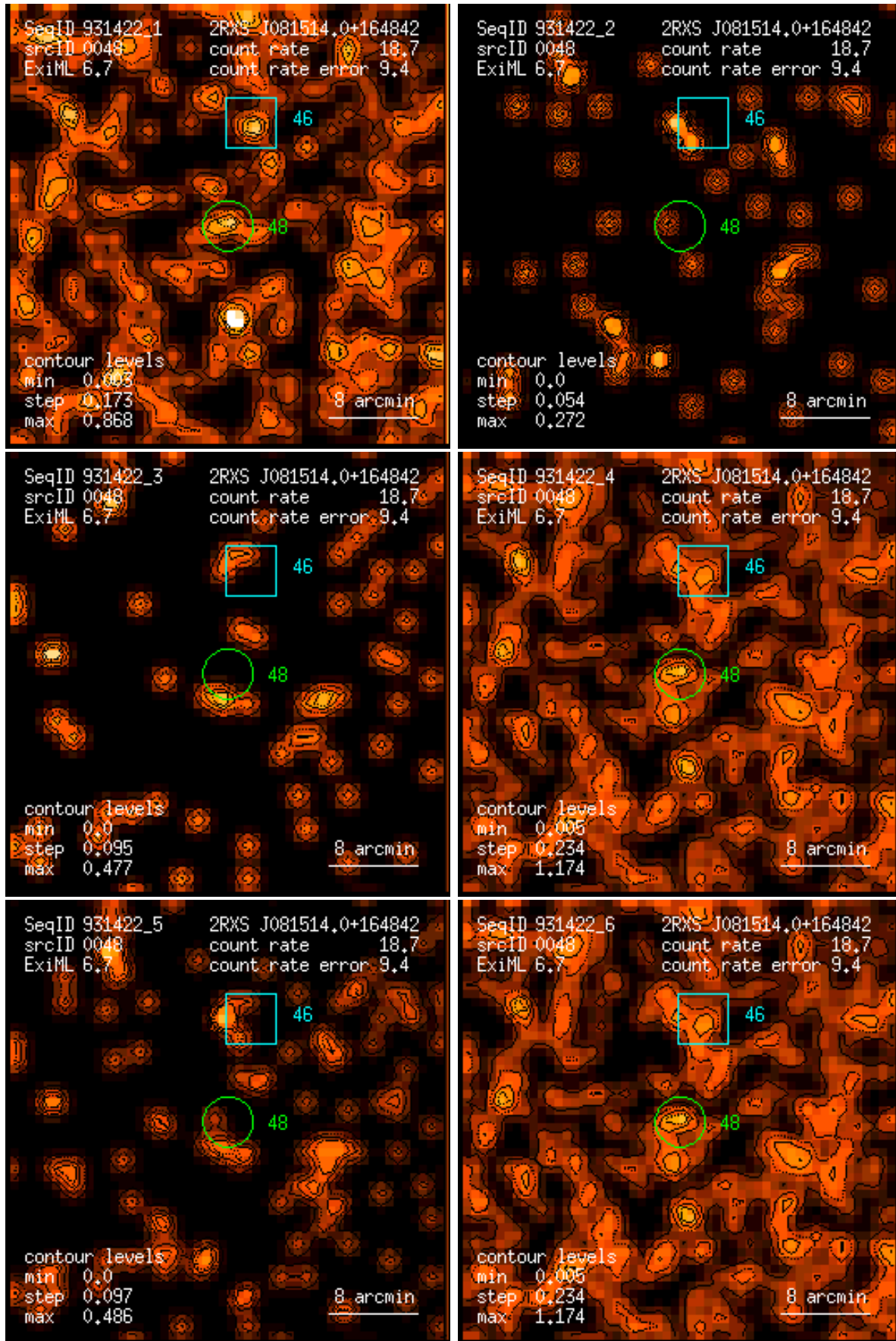
Figure 48: RASS 931422: detection 0048: band rate images, Gaussian filter: (1) PSPC channels 11 – 41, (2) 52 – 90, (3) 91 – 201, (4) 11 – 235, (5) 52 – 201, (6) 11 – 201. Broad band rates in counts/ks. Band rate contour levels in counts/ks/arcmin 2 .
