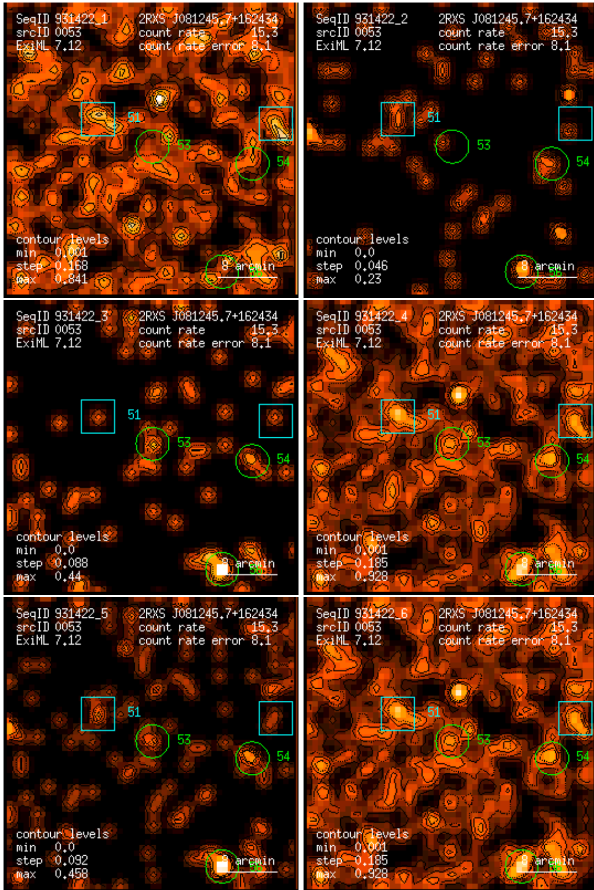
Figure 53: RASS 931422: detection 0053: band rate images, Gaussian filter: (1) PSPC channels 11 – 41, (2) 52 – 90, (3) 91 – 201, (4) 11 – 235, (5) 52 – 201, (6) 11 – 201. Broad band rates in counts/ks. Band rate contour levels in counts/ks/arcmin 2 .
