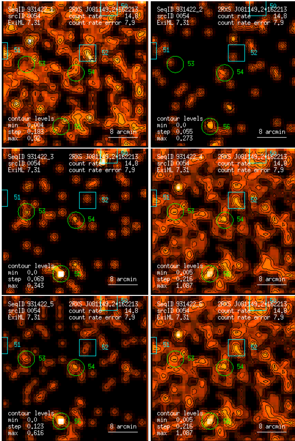
Figure 54: RASS 931422: detection 0054: band rate images, Gaussian filter: (1) PSPC channels 11 – 41, (2) 52 – 90, (3) 91 – 201, (4) 11 – 235, (5) 52 – 201, (6) 11 – 201. Broad band rates in counts/ks. Band rate contour levels in counts/ks/arcmin 2 .
