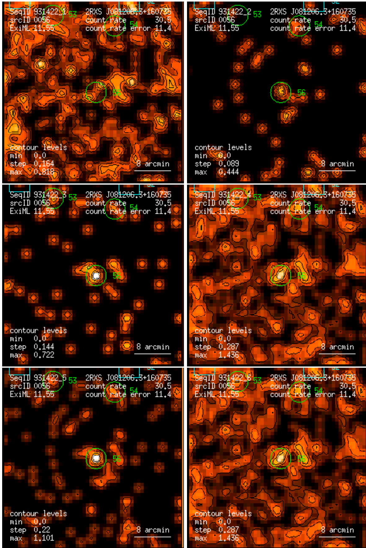
Figure 56: RASS 931422: detection 0056: band rate images, Gaussian filter: (1) PSPC channels 11 – 41, (2) 52 – 90, (3) 91 – 201, (4) 11 – 235, (5) 52 – 201, (6) 11 – 201. Broad band rates in counts/ks. Band rate contour levels in counts/ks/arcmin 2 .
