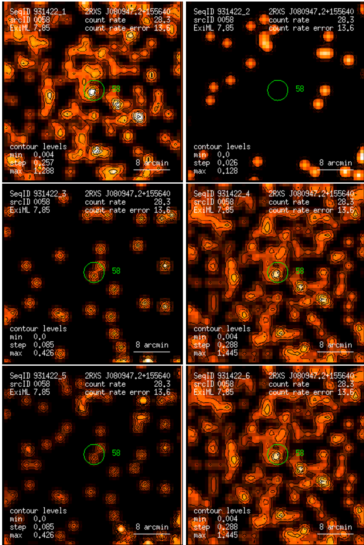
Figure 58: RASS 931422: detection 0058: band rate images, Gaussian filter: (1) PSPC channels 11 – 41, (2) 52 – 90, (3) 91 – 201, (4) 11 – 235, (5) 52 – 201, (6) 11 – 201. Broad band rates in counts/ks. Band rate contour levels in counts/ks/arcmin 2 .
