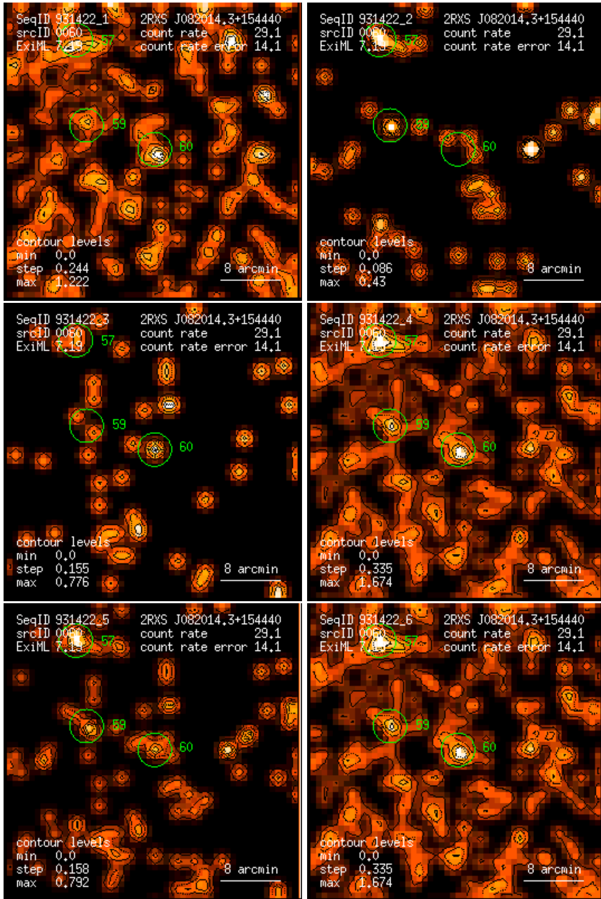
Figure 60: RASS 931422: detection 0060: band rate images, Gaussian filter: (1) PSPC channels 11 – 41, (2) 52 – 90, (3) 91 – 201, (4) 11 – 235, (5) 52 – 201, (6) 11 – 201. Broad band rates in counts/ks. Band rate contour levels in counts/ks/arcmin 2 .
