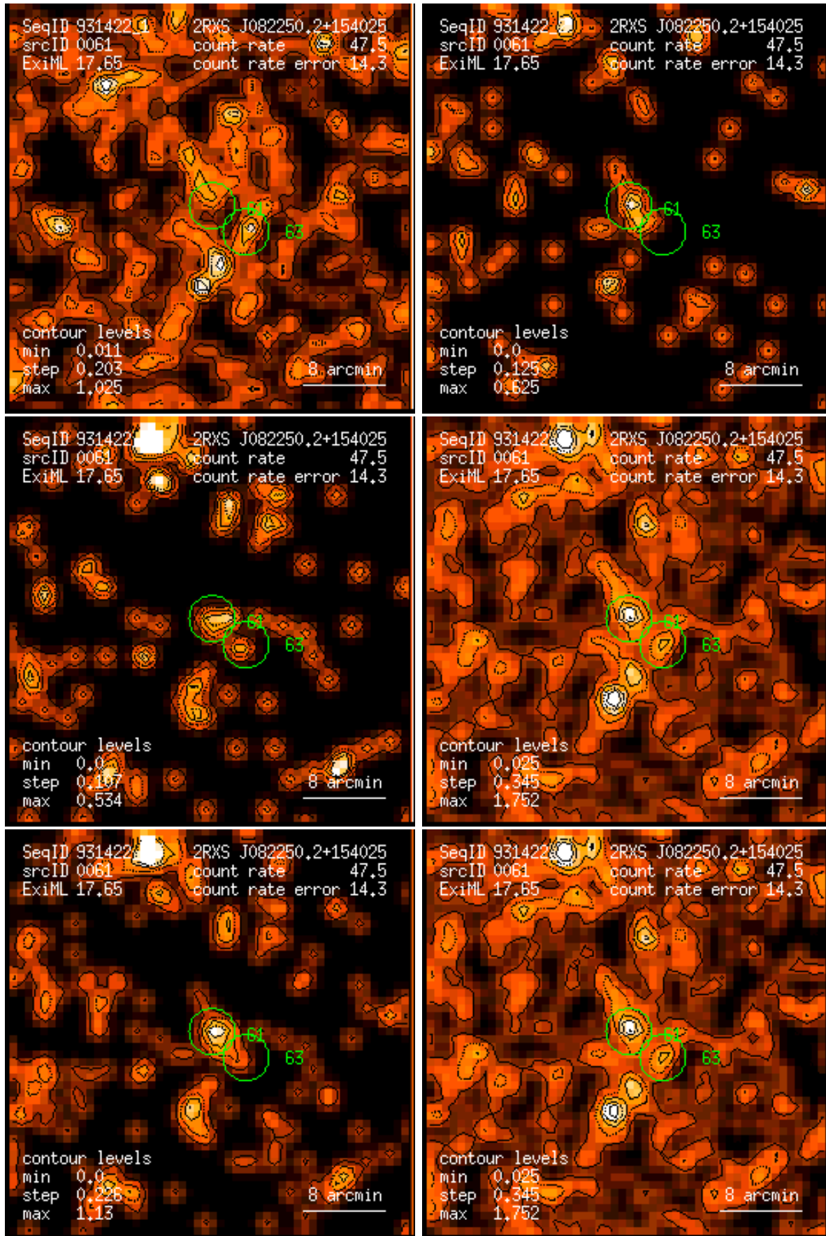
Figure 61: RASS 931422: detection 0061: band rate images, Gaussian filter: (1) PSPC channels 11 – 41, (2) 52 – 90, (3) 91 – 201, (4) 11 – 235, (5) 52 – 201, (6) 11 – 201. Broad band rates in counts/ks. Band rate contour levels in counts/ks/arcmin 2 .
