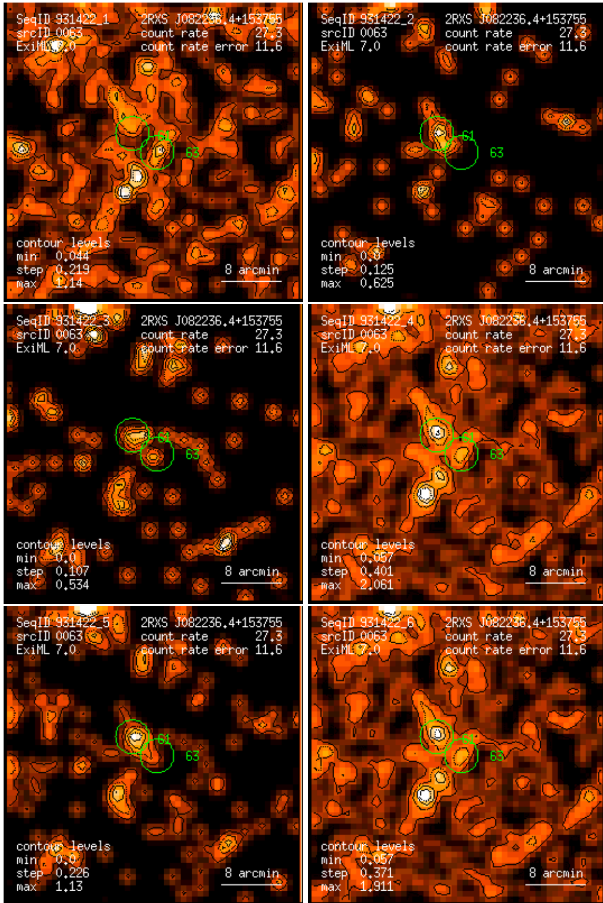
Figure 63: RASS 931422: detection 0063: band rate images, Gaussian filter: (1) PSPC channels 11 – 41, (2) 52 – 90, (3) 91 – 201, (4) 11 – 235, (5) 52 – 201, (6) 11 – 201. Broad band rates in counts/ks. Band rate contour levels in counts/ks/arcmin 2 .
