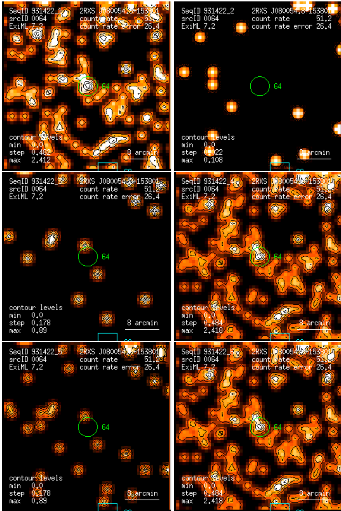
Figure 64: RASS 931422: detection 0064: band rate images, Gaussian filter: (1) PSPC channels 11 – 41, (2) 52 – 90, (3) 91 – 201, (4) 11 – 235, (5) 52 – 201, (6) 11 – 201. Broad band rates in counts/ks. Band rate contour levels in counts/ks/arcmin 2 .
