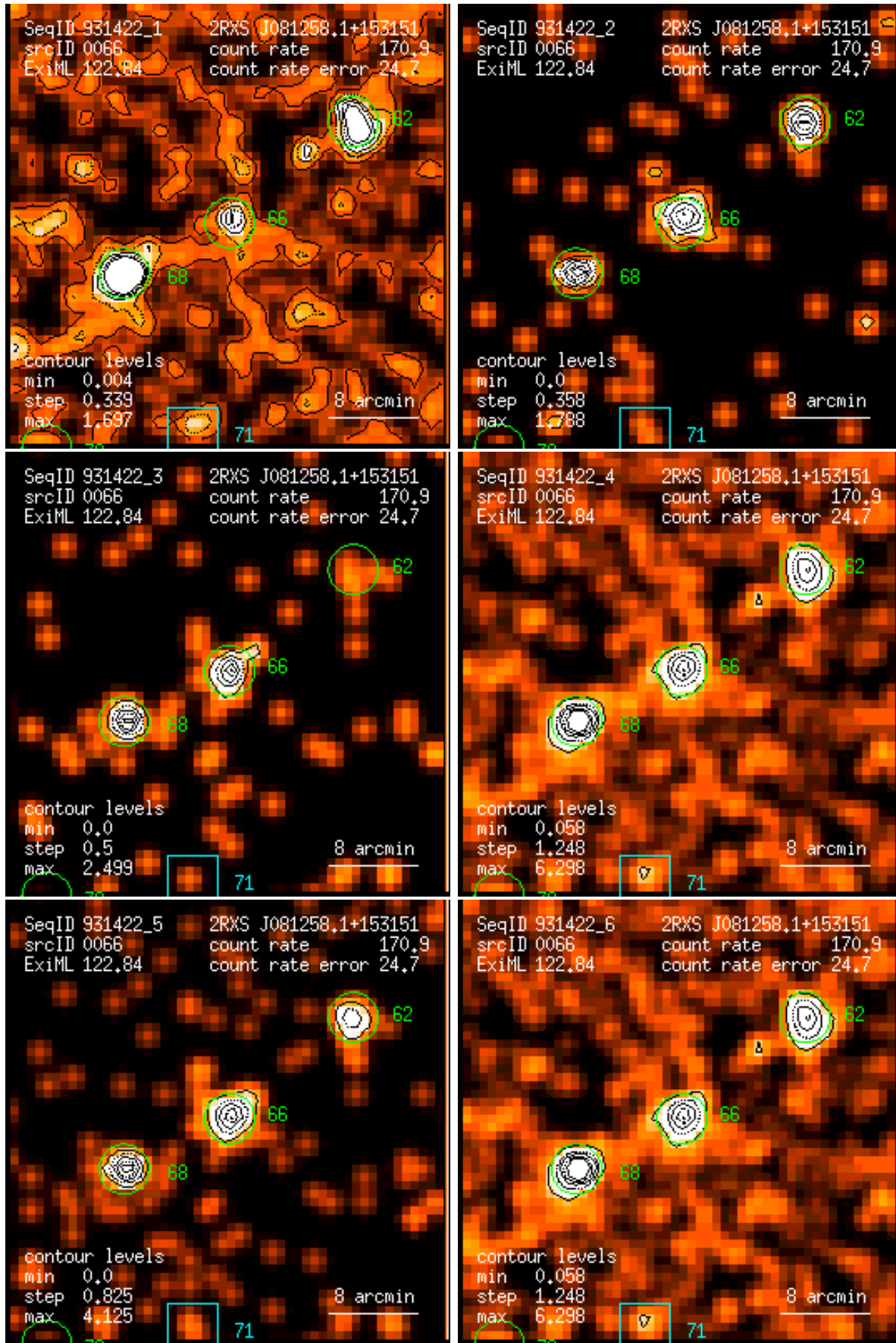
Figure 66: RASS 931422: detection 0066: band rate images, Gaussian filter: (1) PSPC channels 11 – 41, (2) 52 – 90, (3) 91 – 201, (4) 11 – 235, (5) 52 – 201, (6) 11 – 201. Broad band rates in counts/ks. Band rate contour levels in counts/ks/arcmin 2 .
