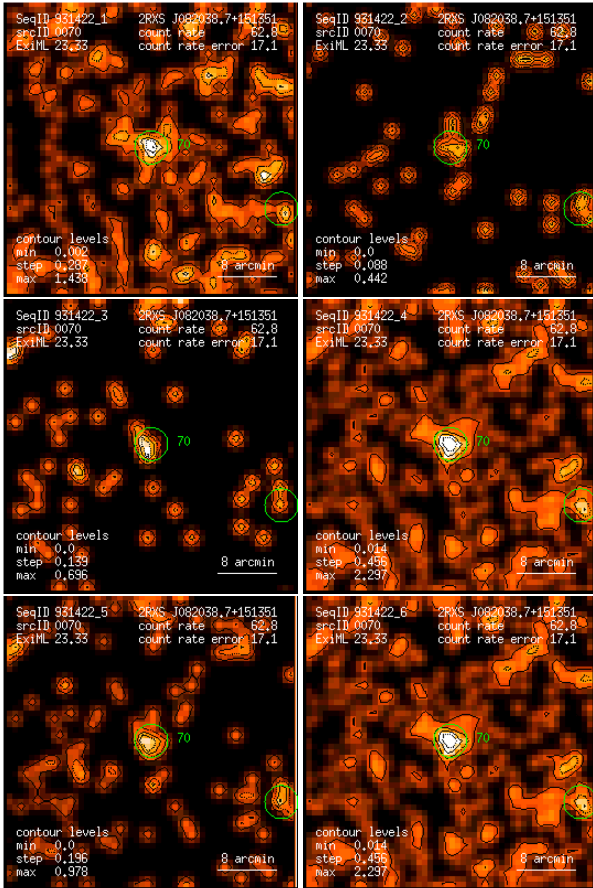
Figure 70: RASS 931422: detection 0070: band rate images, Gaussian filter: (1) PSPC channels 11 – 41, (2) 52 – 90, (3) 91 – 201, (4) 11 – 235, (5) 52 – 201, (6) 11 – 201. Broad band rates in counts/ks. Band rate contour levels in counts/ks/arcmin 2 .
