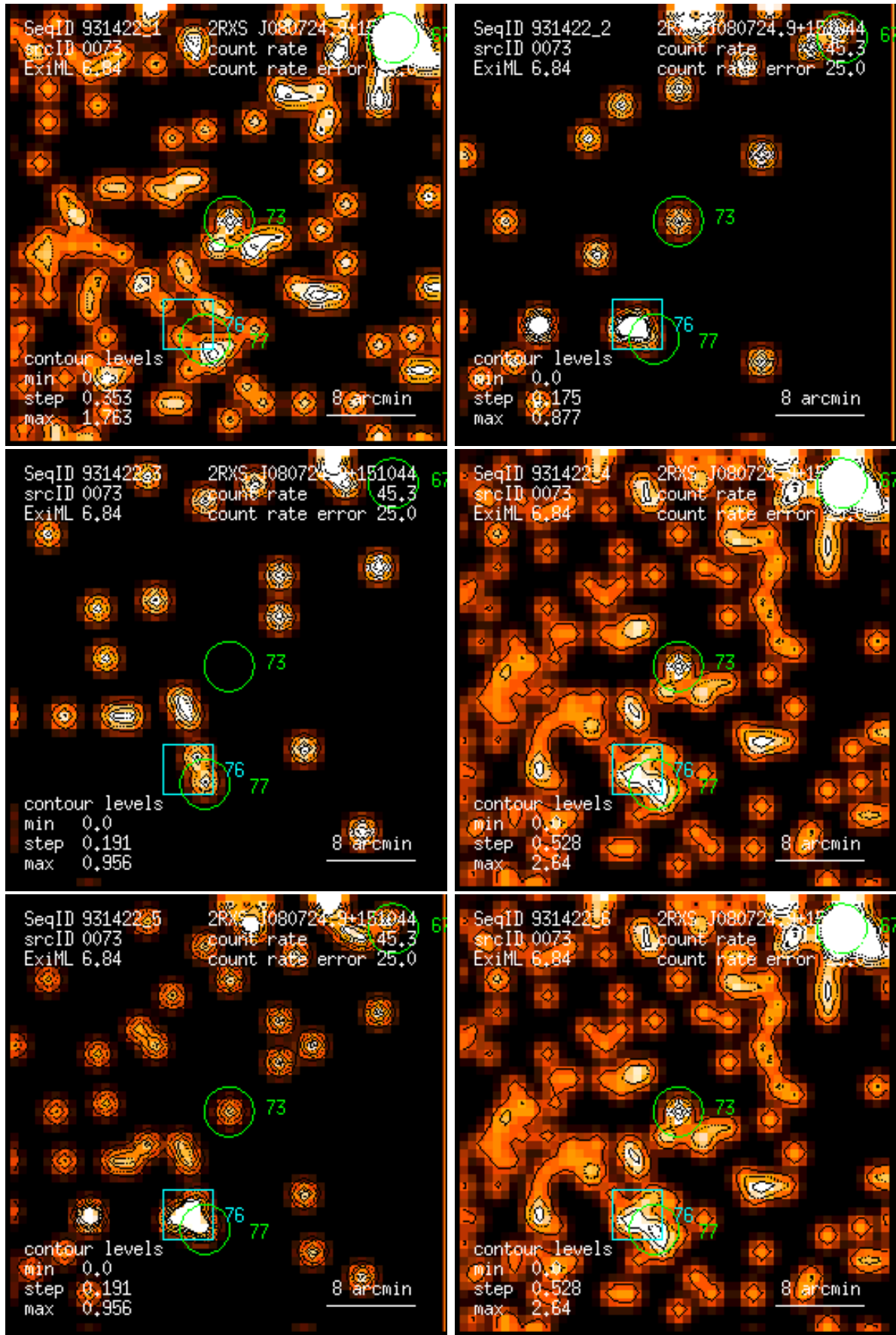
Figure 73: RASS 931422: detection 0073: band rate images, Gaussian filter: (1) PSPC channels 11 – 41, (2) 52 – 90, (3) 91 – 201, (4) 11 – 235, (5) 52 – 201, (6) 11 – 201. Broad band rates in counts/ks. Band rate contour levels in counts/ks/arcmin 2 .
