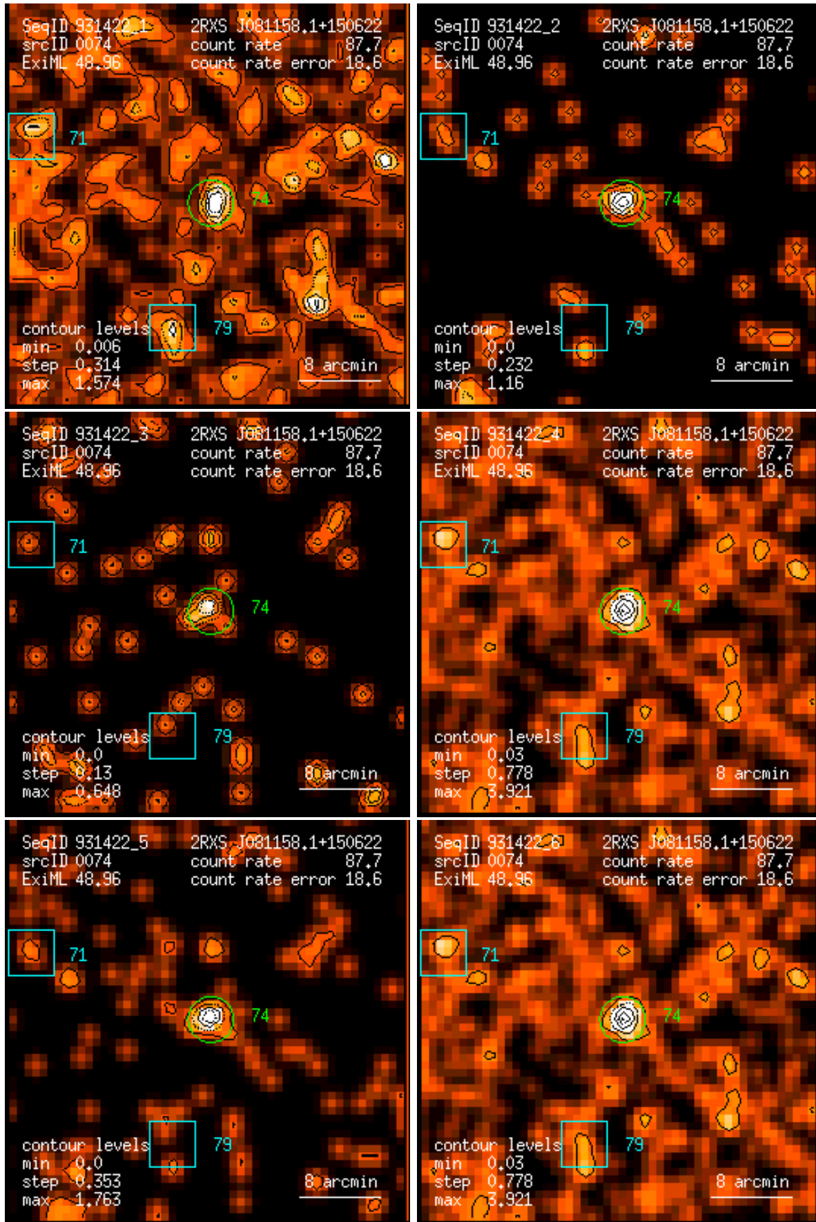
Figure 74: RASS 931422: detection 0074: band rate images, Gaussian filter: (1) PSPC channels 11 – 41, (2) 52 – 90, (3) 91 – 201, (4) 11 – 235, (5) 52 – 201, (6) 11 – 201. Broad band rates in counts/ks. Band rate contour levels in counts/ks/arcmin 2 .
