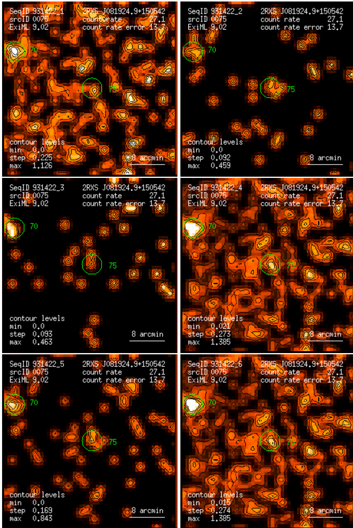
Figure 75: RASS 931422: detection 0075: band rate images, Gaussian filter: (1) PSPC channels 11 – 41, (2) 52 – 90, (3) 91 – 201, (4) 11 – 235, (5) 52 – 201, (6) 11 – 201. Broad band rates in counts/ks. Band rate contour levels in counts/ks/arcmin 2 .
