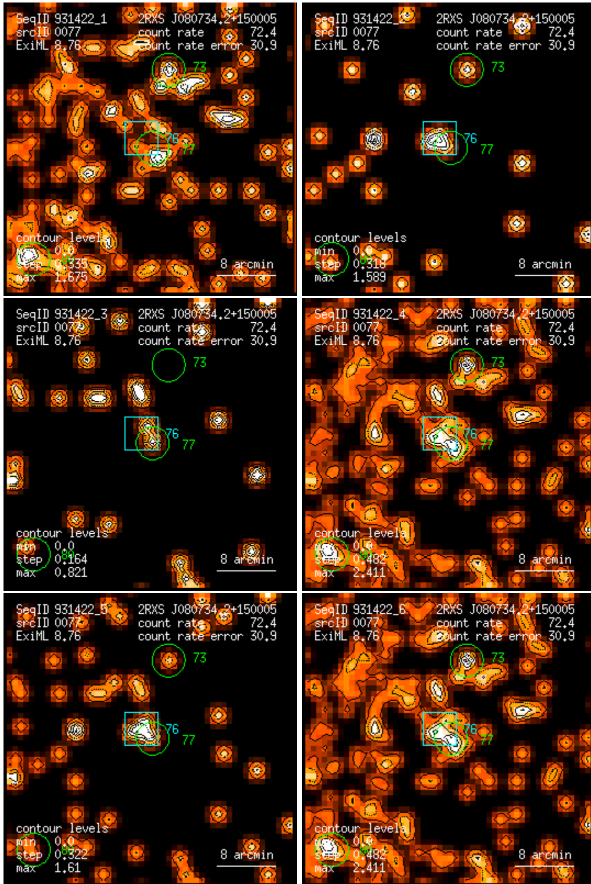
Figure 77: RASS 931422: detection 0077: band rate images, Gaussian filter: (1) PSPC channels 11 – 41, (2) 52 – 90, (3) 91 – 201, (4) 11 – 235, (5) 52 – 201, (6) 11 – 201. Broad band rates in counts/ks. Band rate contour levels in counts/ks/arcmin 2 .
