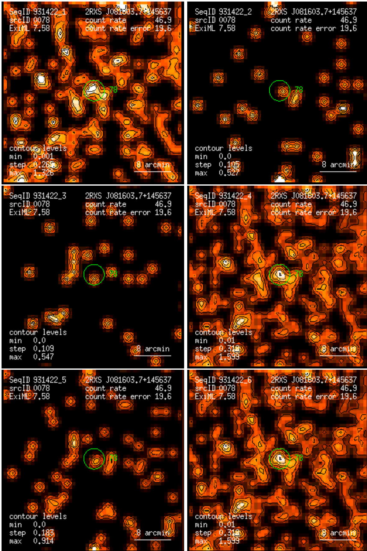
Figure 78: RASS 931422: detection 0078: band rate images, Gaussian filter: (1) PSPC channels 11 – 41, (2) 52 – 90, (3) 91 – 201, (4) 11 – 235, (5) 52 – 201, (6) 11 – 201. Broad band rates in counts/ks. Band rate contour levels in counts/ks/arcmin 2 .
