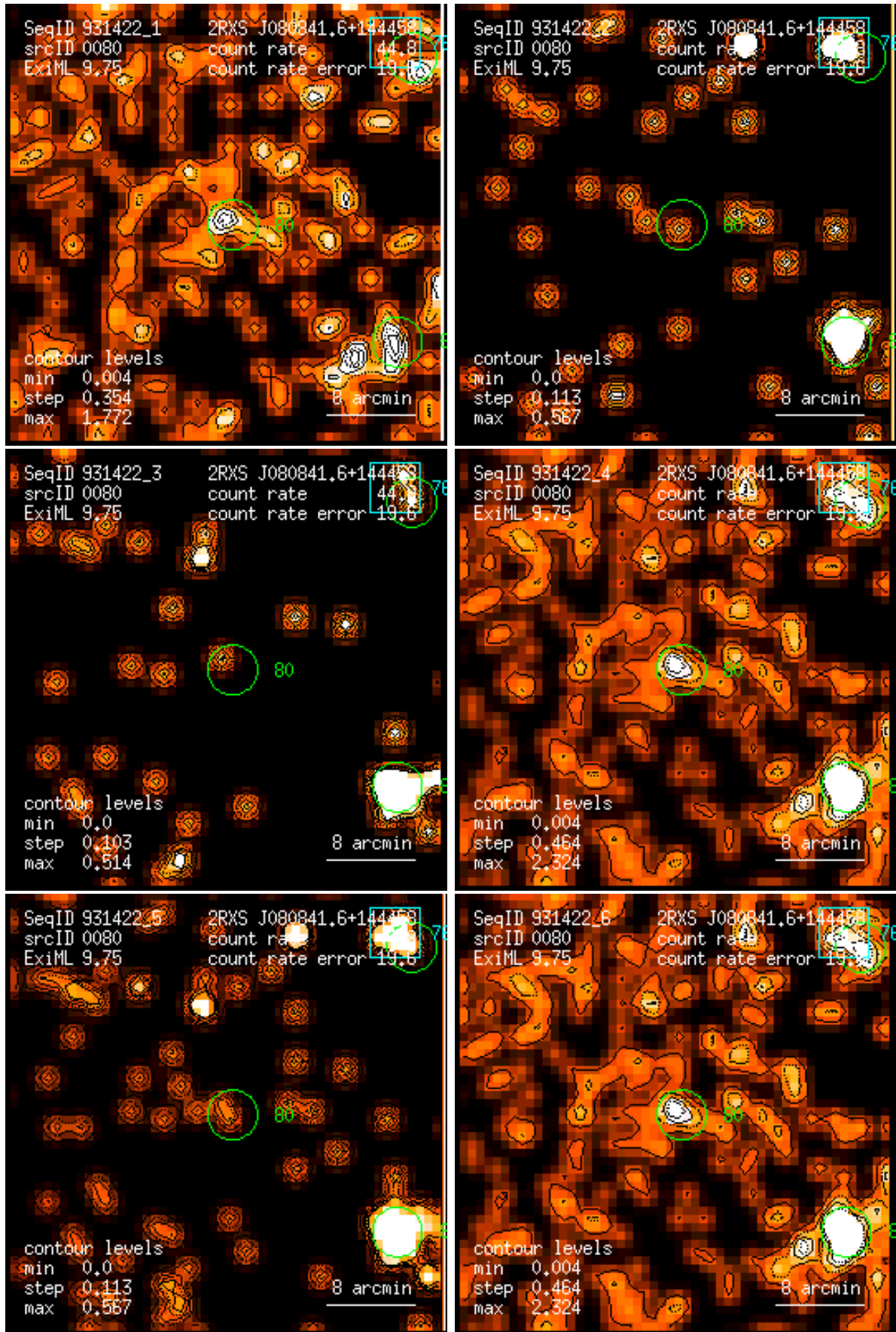
Figure 80: RASS 931422: detection 0080: band rate images, Gaussian filter: (1) PSPC channels 11 – 41, (2) 52 – 90, (3) 91 – 201, (4) 11 – 235, (5) 52 – 201, (6) 11 – 201. Broad band rates in counts/ks. Band rate contour levels in counts/ks/arcmin 2 .
