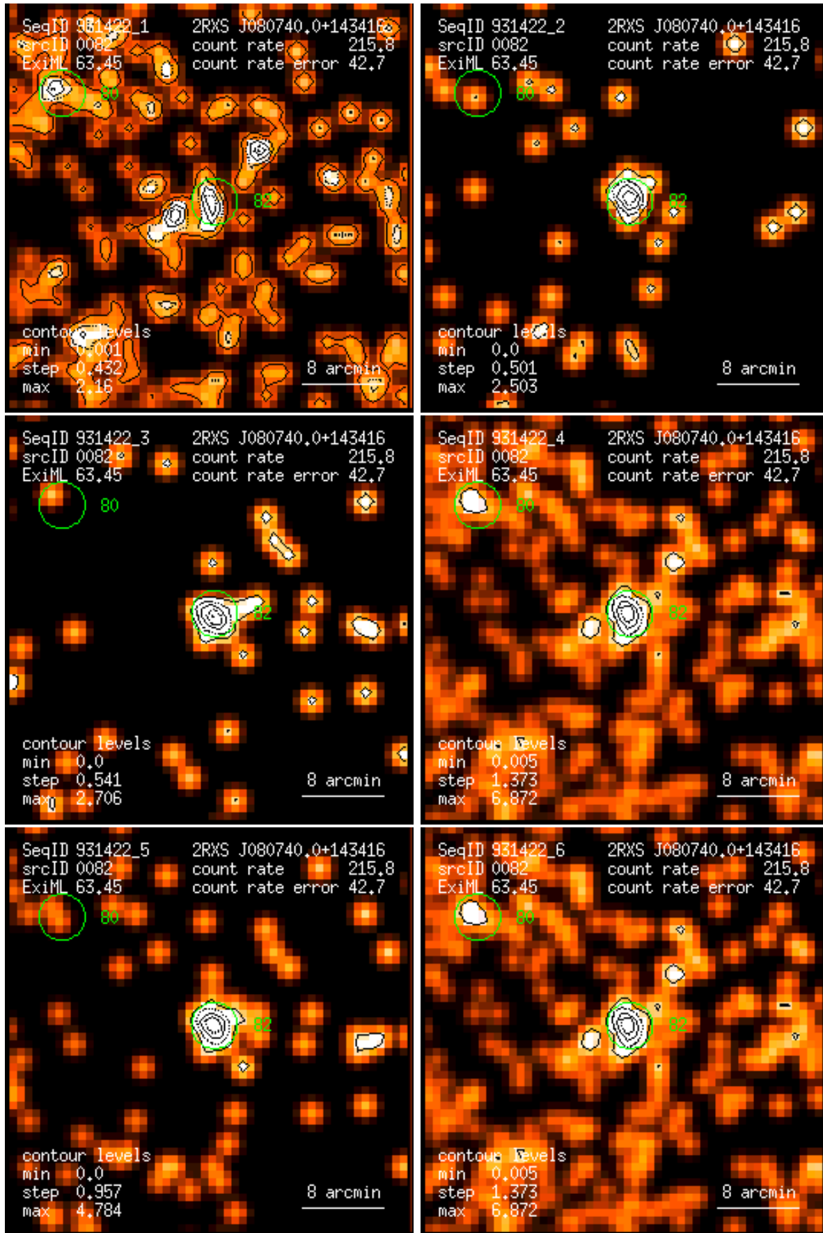
Figure 82: RASS 931422: detection 0082: band rate images, Gaussian filter: (1) PSPC channels 11 – 41, (2) 52 – 90, (3) 91 – 201, (4) 11 – 235, (5) 52 – 201, (6) 11 – 201. Broad band rates in counts/ks. Band rate contour levels in counts/ks/arcmin 2 .
