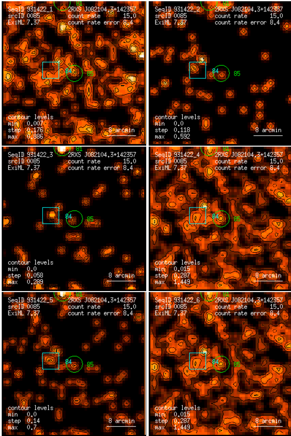
Figure 85: RASS 931422: detection 0085: band rate images, Gaussian filter: (1) PSPC channels 11 – 41, (2) 52 – 90, (3) 91 – 201, (4) 11 – 235, (5) 52 – 201, (6) 11 – 201. Broad band rates in counts/ks. Band rate contour levels in counts/ks/arcmin 2 .
