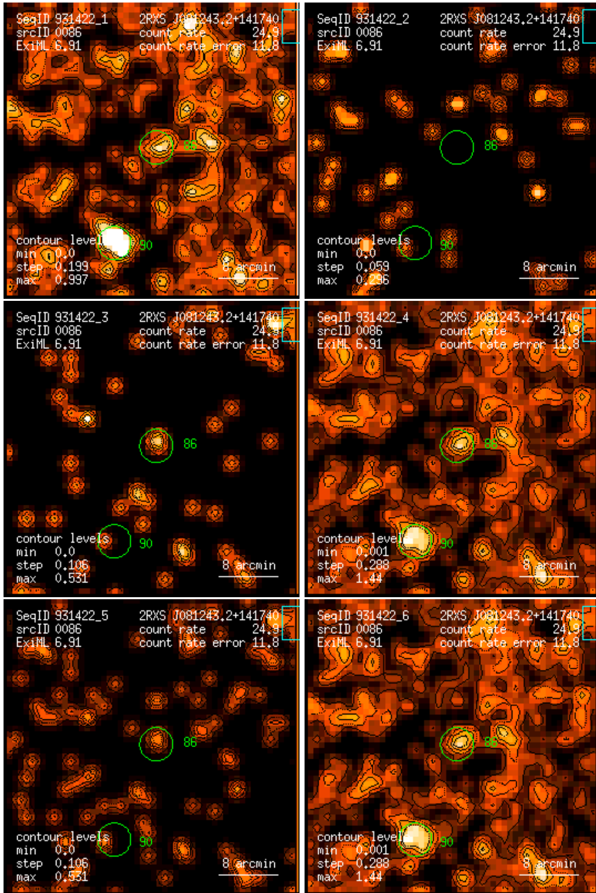
Figure 86: RASS 931422: detection 0086: band rate images, Gaussian filter: (1) PSPC channels 11 – 41, (2) 52 – 90, (3) 91 – 201, (4) 11 – 235, (5) 52 – 201, (6) 11 – 201. Broad band rates in counts/ks. Band rate contour levels in counts/ks/arcmin 2 .
