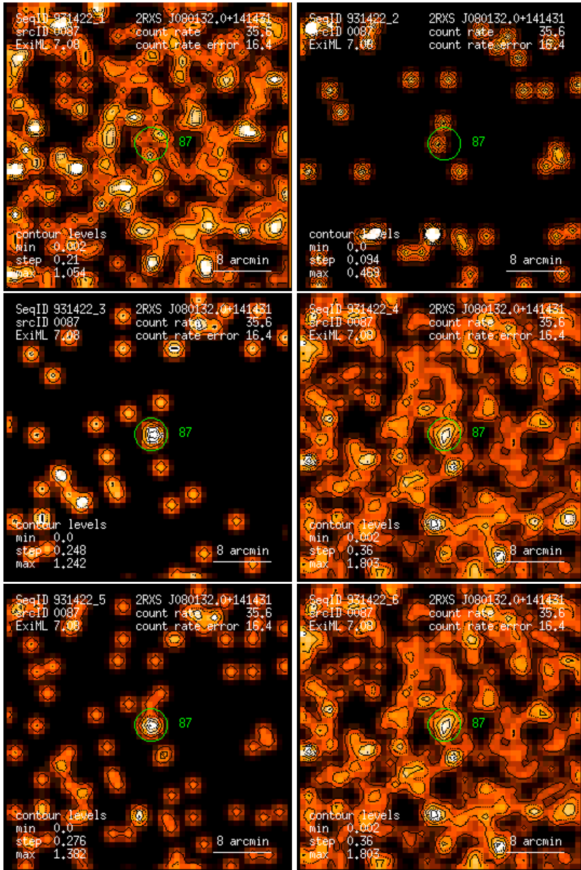
Figure 87: RASS 931422: detection 0087: band rate images, Gaussian filter: (1) PSPC channels 11 – 41, (2) 52 – 90, (3) 91 – 201, (4) 11 – 235, (5) 52 – 201, (6) 11 – 201. Broad band rates in counts/ks. Band rate contour levels in counts/ks/arcmin 2 .
