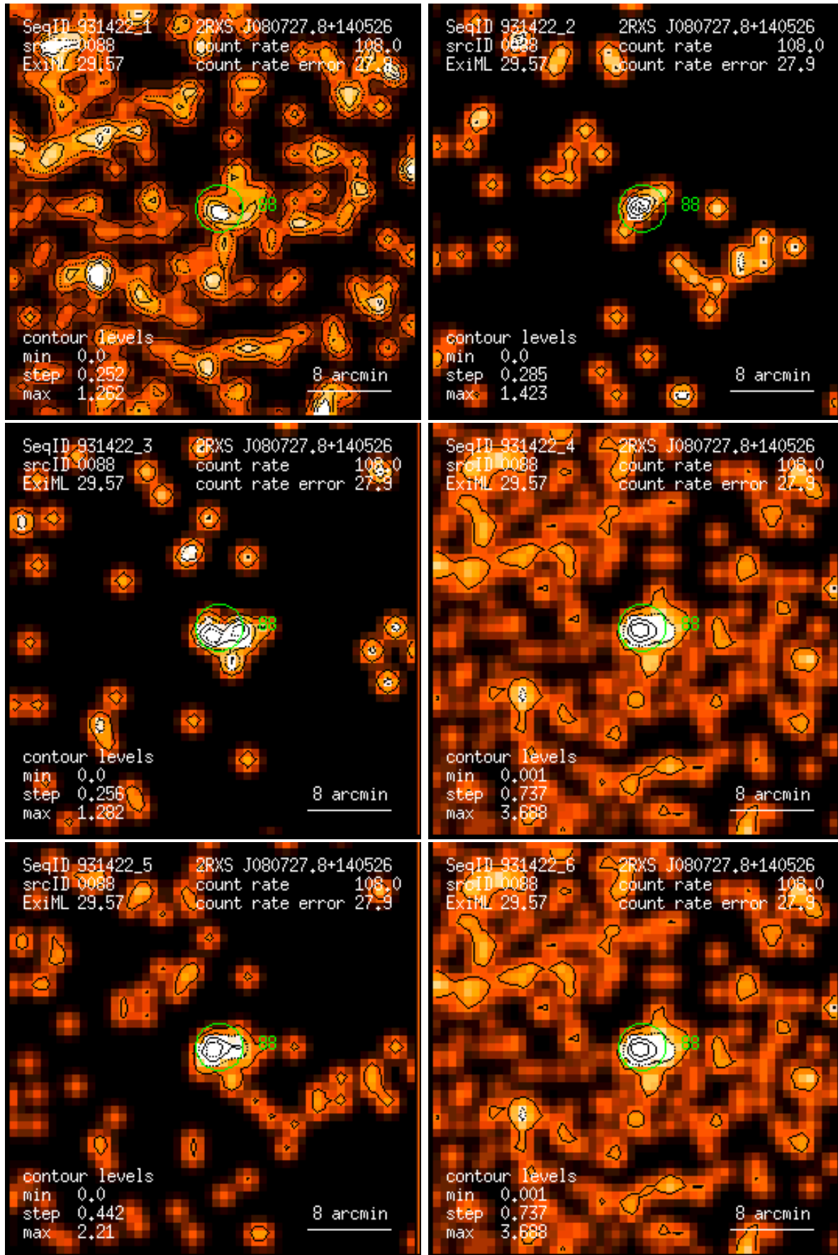
Figure 88: RASS 931422: detection 0088: band rate images, Gaussian filter: (1) PSPC channels 11 – 41, (2) 52 – 90, (3) 91 – 201, (4) 11 – 235, (5) 52 – 201, (6) 11 – 201. Broad band rates in counts/ks. Band rate contour levels in counts/ks/arcmin 2 .
