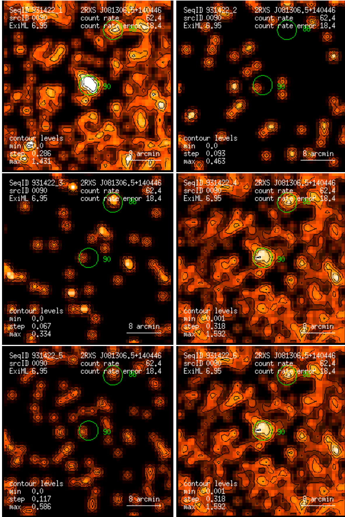
Figure 90: RASS 931422: detection 0090: band rate images, Gaussian filter: (1) PSPC channels 11 – 41, (2) 52 – 90, (3) 91 – 201, (4) 11 – 235, (5) 52 – 201, (6) 11 – 201. Broad band rates in counts/ks. Band rate contour levels in counts/ks/arcmin 2 .
