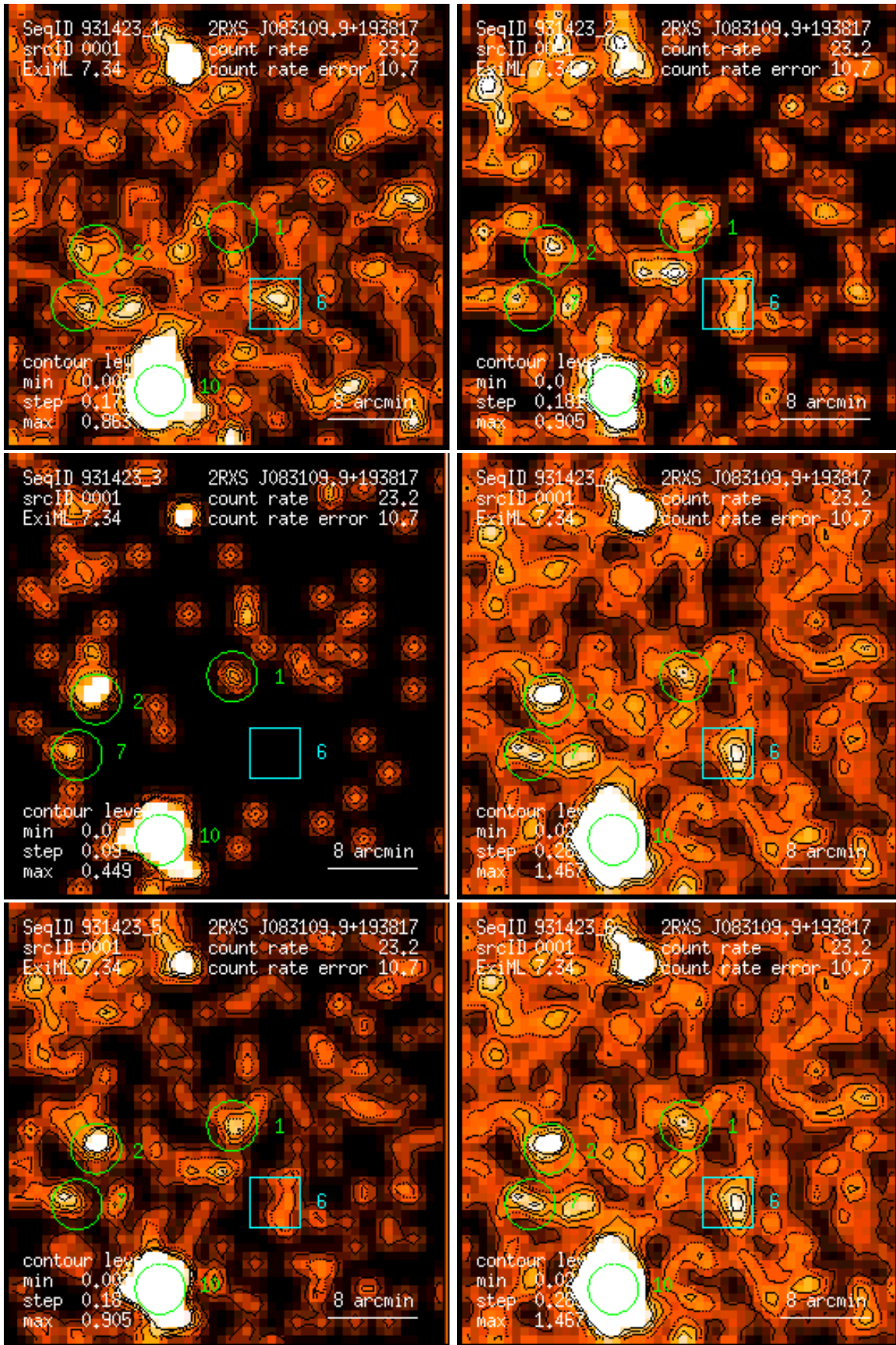
Figure 1: RASS 931423: detection 0001: band rate images, Gaussian filter: (1) PSPC channels 11 – 41, (2) 52 – 90, (3) 91 – 201, (4) 11 – 235, (5) 52 – 201, (6) 11 – 201. Broad band rates in counts/ks. Band rate contour levels in counts/ks/arcmin 2 .
