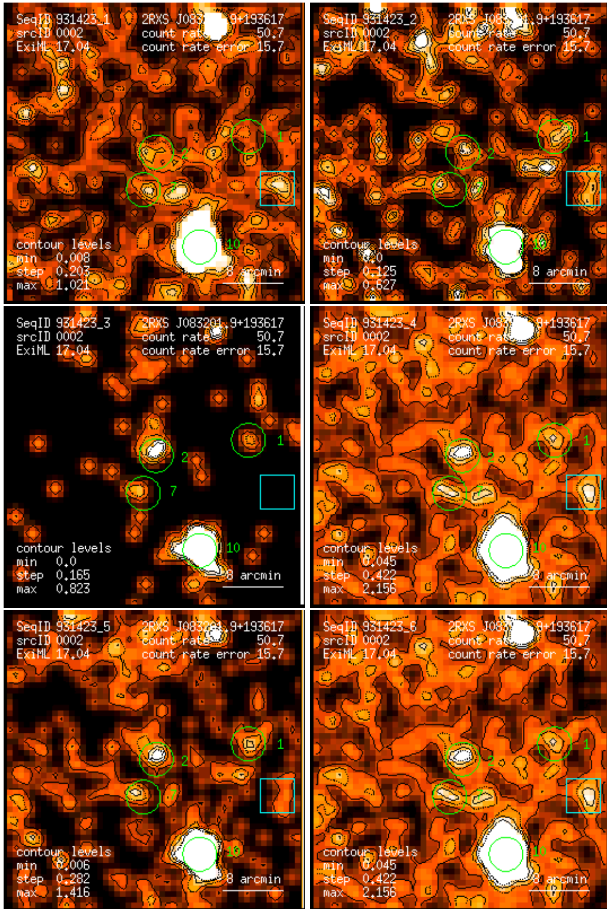
Figure 2: RASS 931423: detection 0002: band rate images, Gaussian filter: (1) PSPC channels 11 – 41, (2) 52 – 90, (3) 91 – 201, (4) 11 – 235, (5) 52 – 201, (6) 11 – 201. Broad band rates in counts/ks. Band rate contour levels in counts/ks/arcmin 2 .
