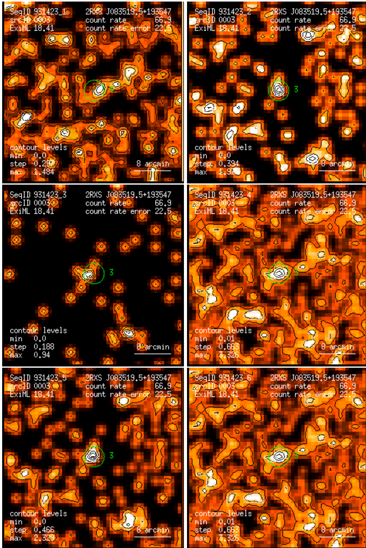
Figure 3: RASS 931423: detection 0003: band rate images, Gaussian filter: (1) PSPC channels 11 – 41, (2) 52 – 90, (3) 91 – 201, (4) 11 – 235, (5) 52 – 201, (6) 11 – 201. Broad band rates in counts/ks. Band rate contour levels in counts/ks/arcmin 2 .
