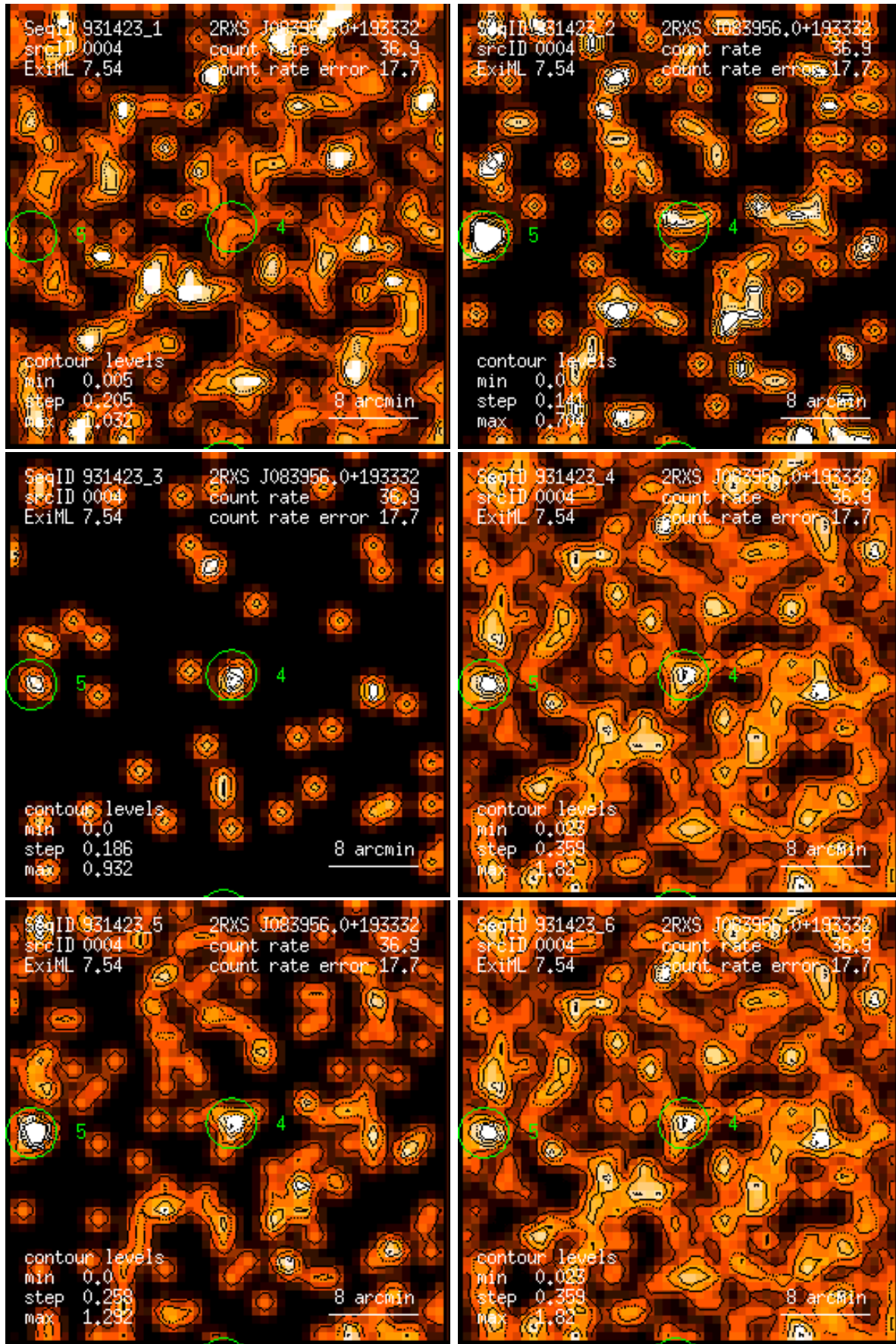
Figure 4: RASS 931423: detection 0004: band rate images, Gaussian filter: (1) PSPC channels 11 – 41, (2) 52 – 90, (3) 91 – 201, (4) 11 – 235, (5) 52 – 201, (6) 11 – 201. Broad band rates in counts/ks. Band rate contour levels in counts/ks/arcmin 2 .
