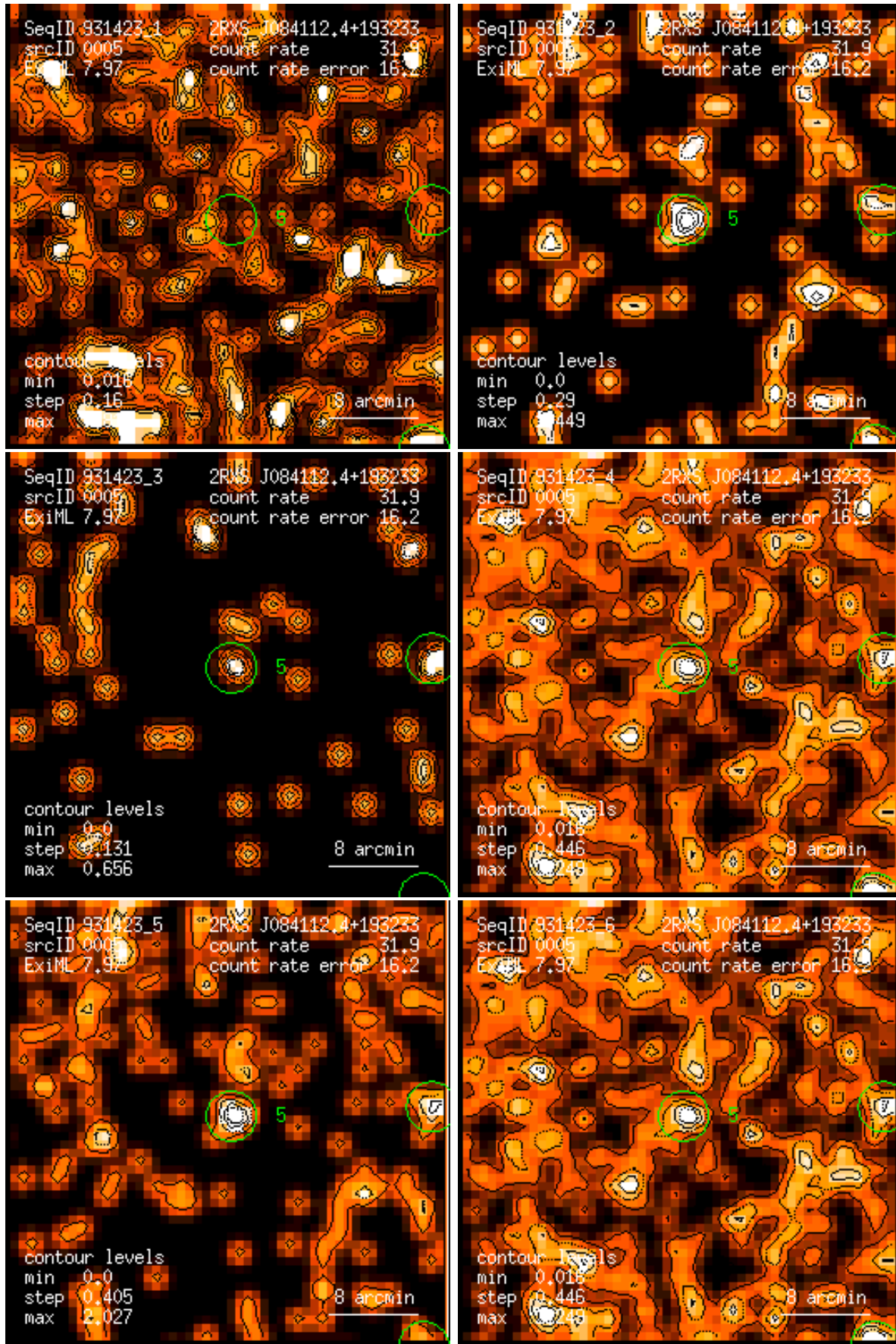
Figure 5: RASS 931423: detection 0005: band rate images, Gaussian filter: (1) PSPC channels 11 – 41, (2) 52 – 90, (3) 91 – 201, (4) 11 – 235, (5) 52 – 201, (6) 11 – 201. Broad band rates in counts/ks. Band rate contour levels in counts/ks/arcmin 2 .
