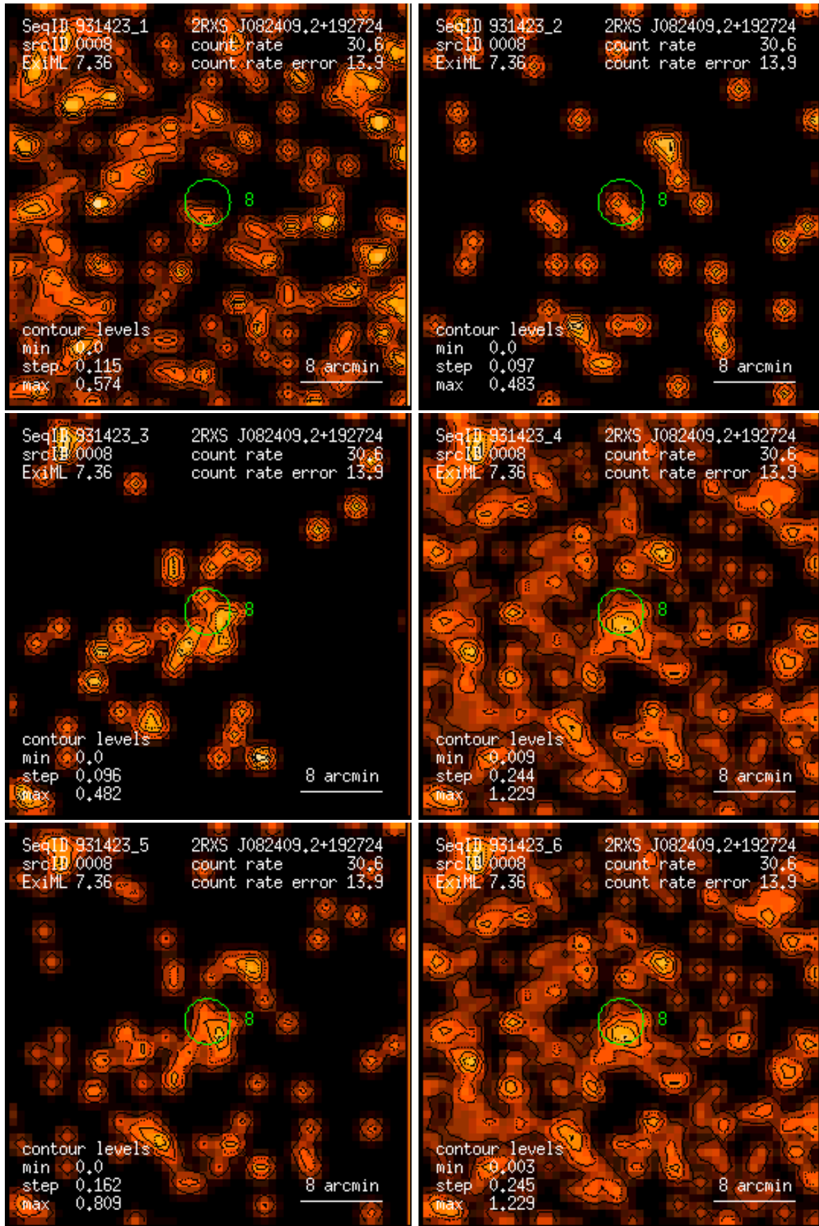
Figure 8: RASS 931423: detection 0008: band rate images, Gaussian filter: (1) PSPC channels 11 – 41, (2) 52 – 90, (3) 91 – 201, (4) 11 – 235, (5) 52 – 201, (6) 11 – 201. Broad band rates in counts/ks. Band rate contour levels in counts/ks/arcmin 2 .
