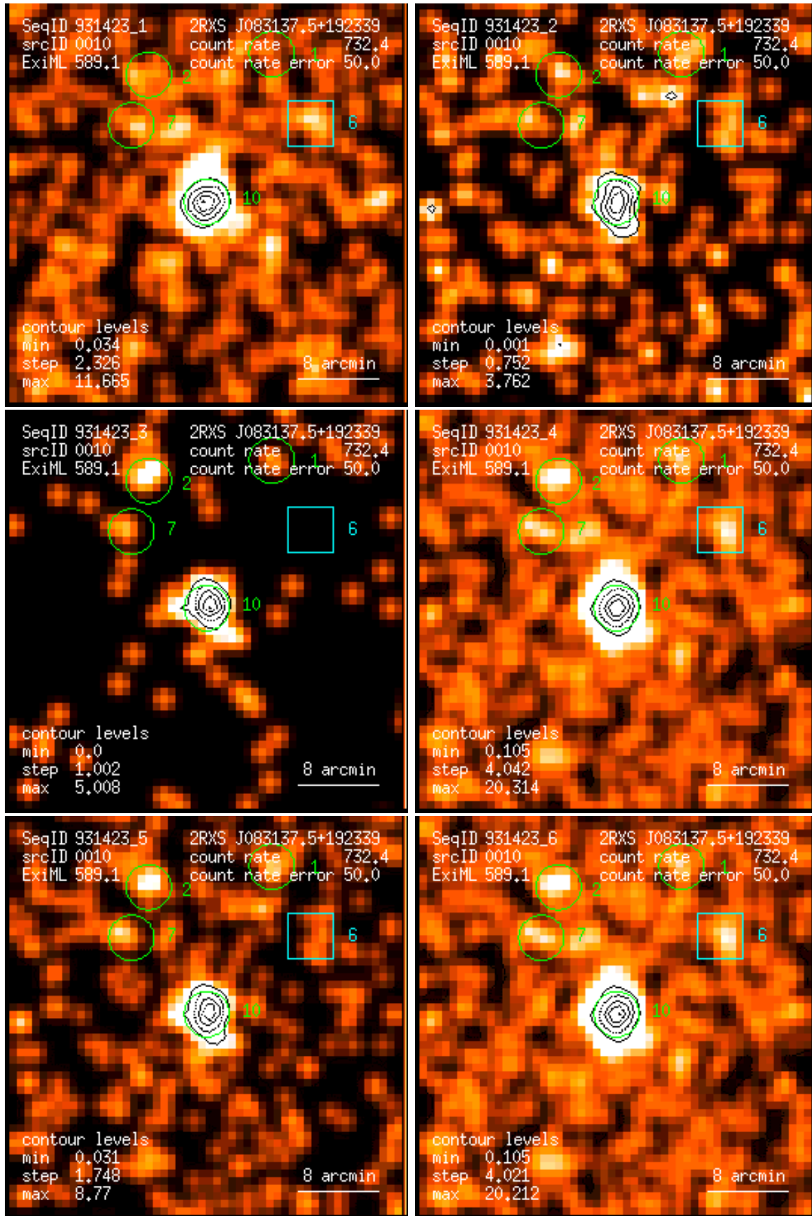
Figure 10: RASS 931423: detection 0010: band rate images, Gaussian filter: (1) PSPC channels 11 – 41, (2) 52 – 90, (3) 91 – 201, (4) 11 – 235, (5) 52 – 201, (6) 11 – 201. Broad band rates in counts/ks. Band rate contour levels in counts/ks/arcmin 2 .
