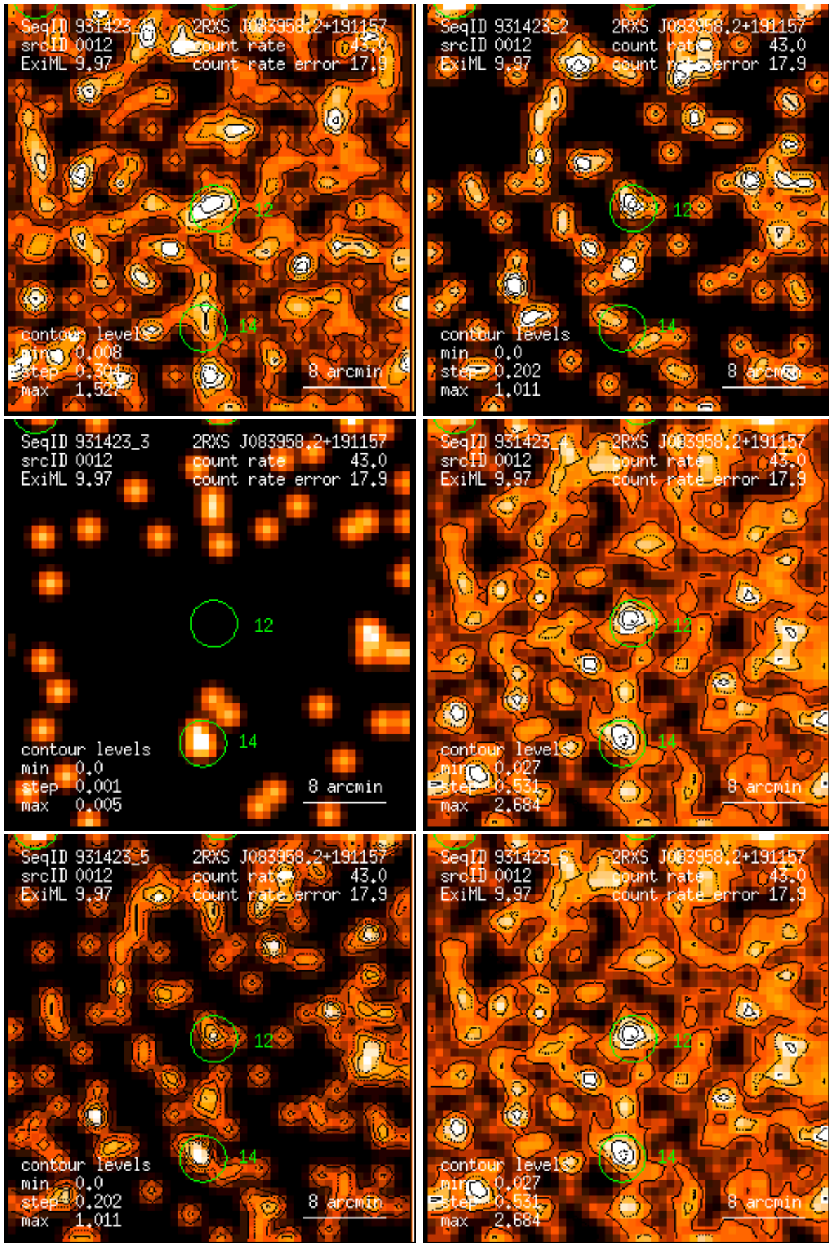
Figure 12: RASS 931423: detection 0012: band rate images, Gaussian filter: (1) PSPC channels 11 – 41, (2) 52 – 90, (3) 91 – 201, (4) 11 – 235, (5) 52 – 201, (6) 11 – 201. Broad band rates in counts/ks. Band rate contour levels in counts/ks/arcmin 2 .
