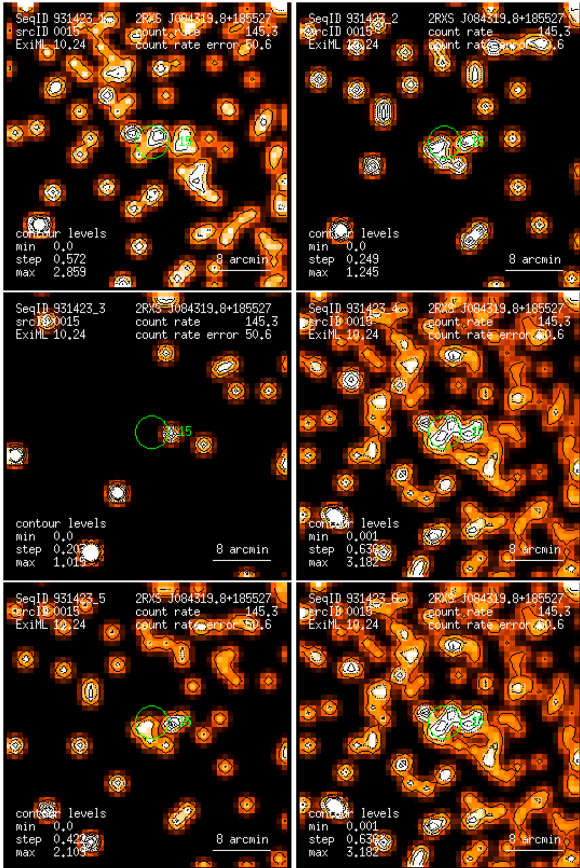
Figure 15: RASS 931423: detection 0015: band rate images, Gaussian filter: (1) PSPC channels 11 – 41, (2) 52 – 90, (3) 91 – 201, (4) 11 – 235, (5) 52 – 201, (6) 11 – 201. Broad band rates in counts/ks. Band rate contour levels in counts/ks/arcmin 2 .
