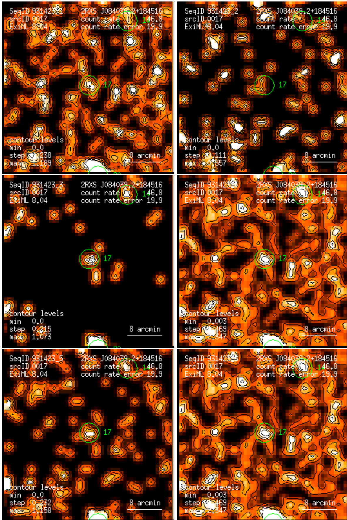
Figure 17: RASS 931423: detection 0017: band rate images, Gaussian filter: (1) PSPC channels 11 – 41, (2) 52 – 90, (3) 91 – 201, (4) 11 – 235, (5) 52 – 201, (6) 11 – 201. Broad band rates in counts/ks. Band rate contour levels in counts/ks/arcmin 2 .
