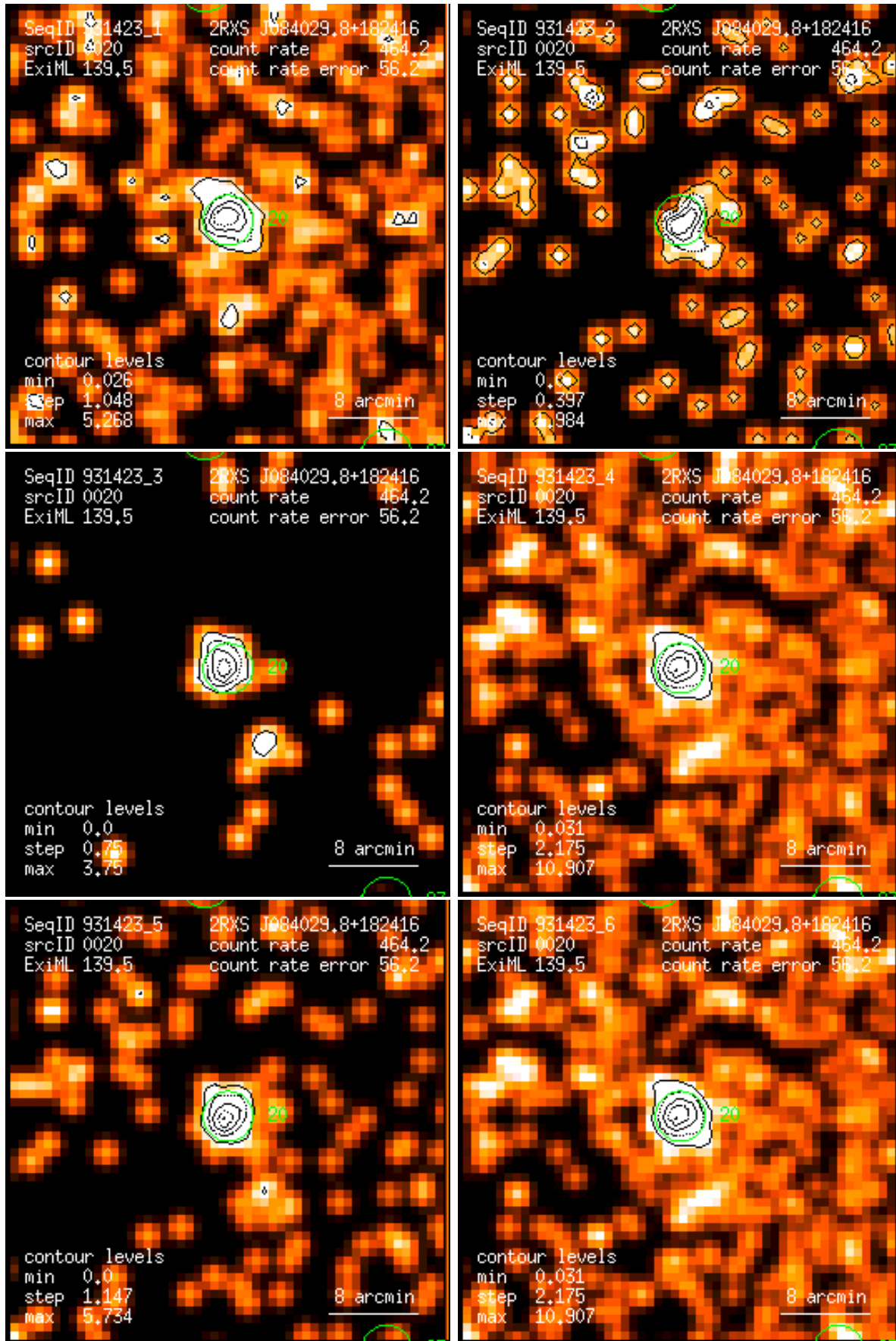
Figure 20: RASS 931423: detection 0020: band rate images, Gaussian filter: (1) PSPC channels 11 – 41, (2) 52 – 90, (3) 91 – 201, (4) 11 – 235, (5) 52 – 201, (6) 11 – 201. Broad band rates in counts/ks. Band rate contour levels in counts/ks/arcmin 2 .
