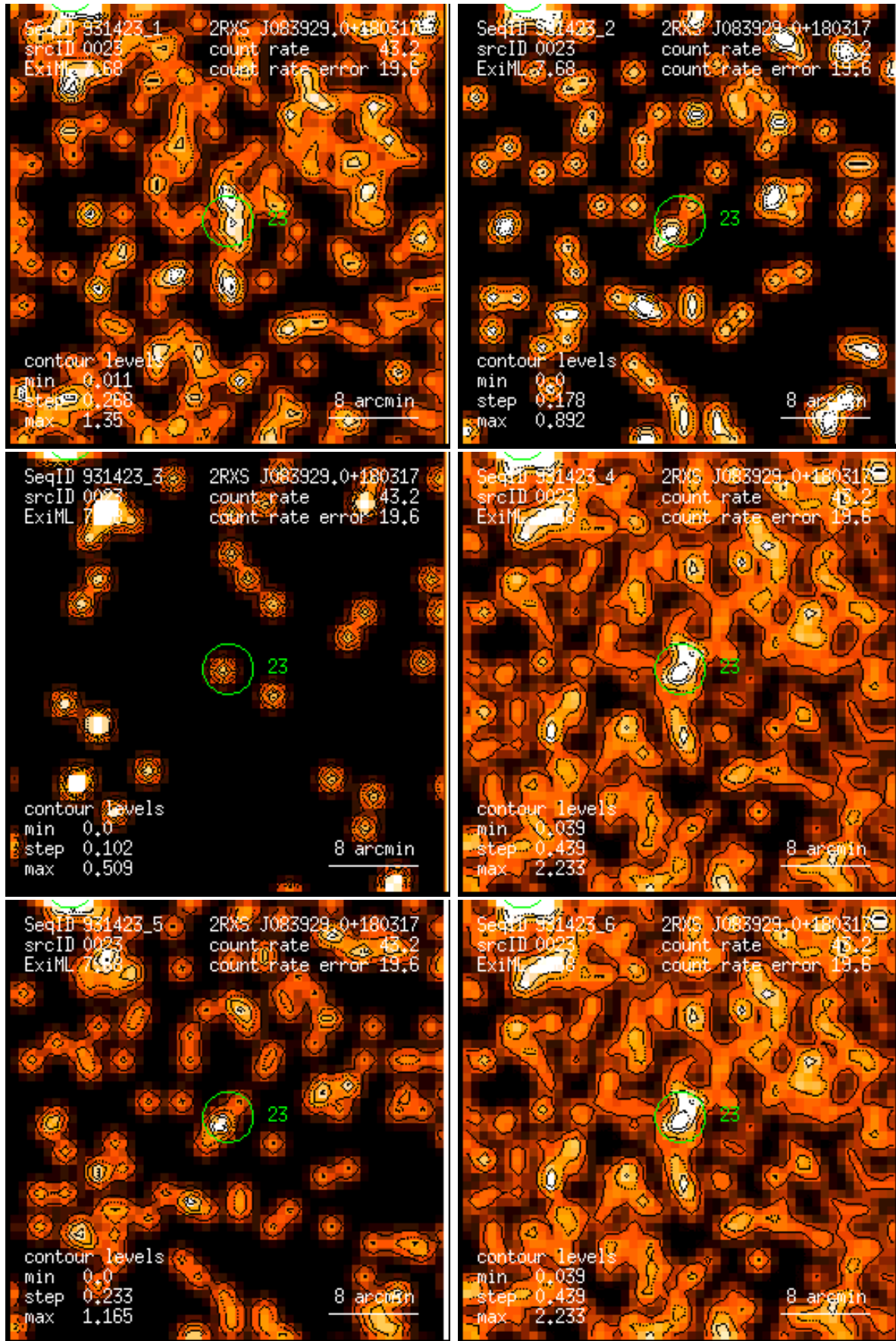
Figure 23: RASS 931423: detection 0023: band rate images, Gaussian filter: (1) PSPC channels 11 – 41, (2) 52 – 90, (3) 91 – 201, (4) 11 – 235, (5) 52 – 201, (6) 11 – 201. Broad band rates in counts/ks. Band rate contour levels in counts/ks/arcmin 2 .
