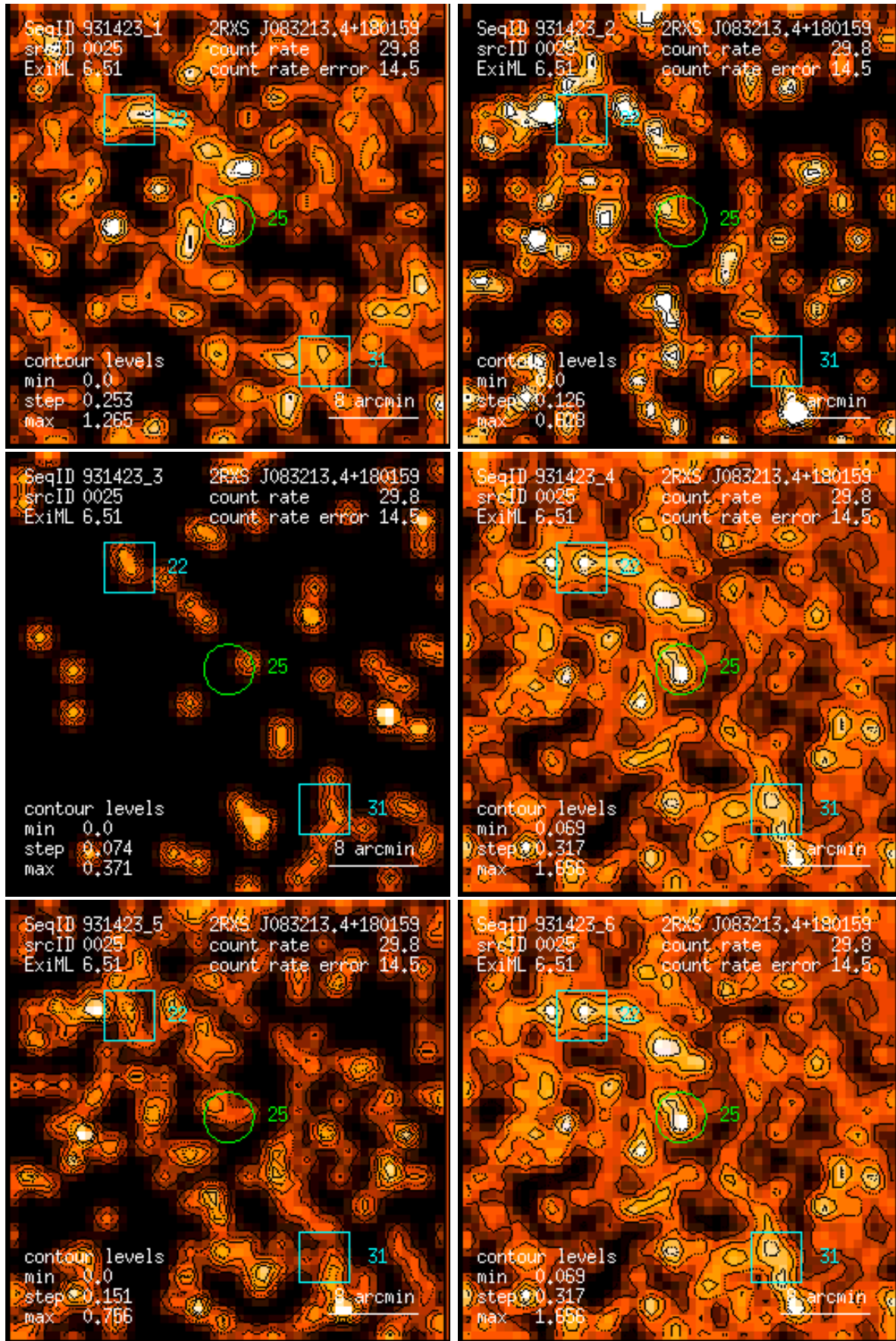
Figure 25: RASS 931423: detection 0025: band rate images, Gaussian filter: (1) PSPC channels 11 – 41, (2) 52 – 90, (3) 91 – 201, (4) 11 – 235, (5) 52 – 201, (6) 11 – 201. Broad band rates in counts/ks. Band rate contour levels in counts/ks/arcmin 2 .
