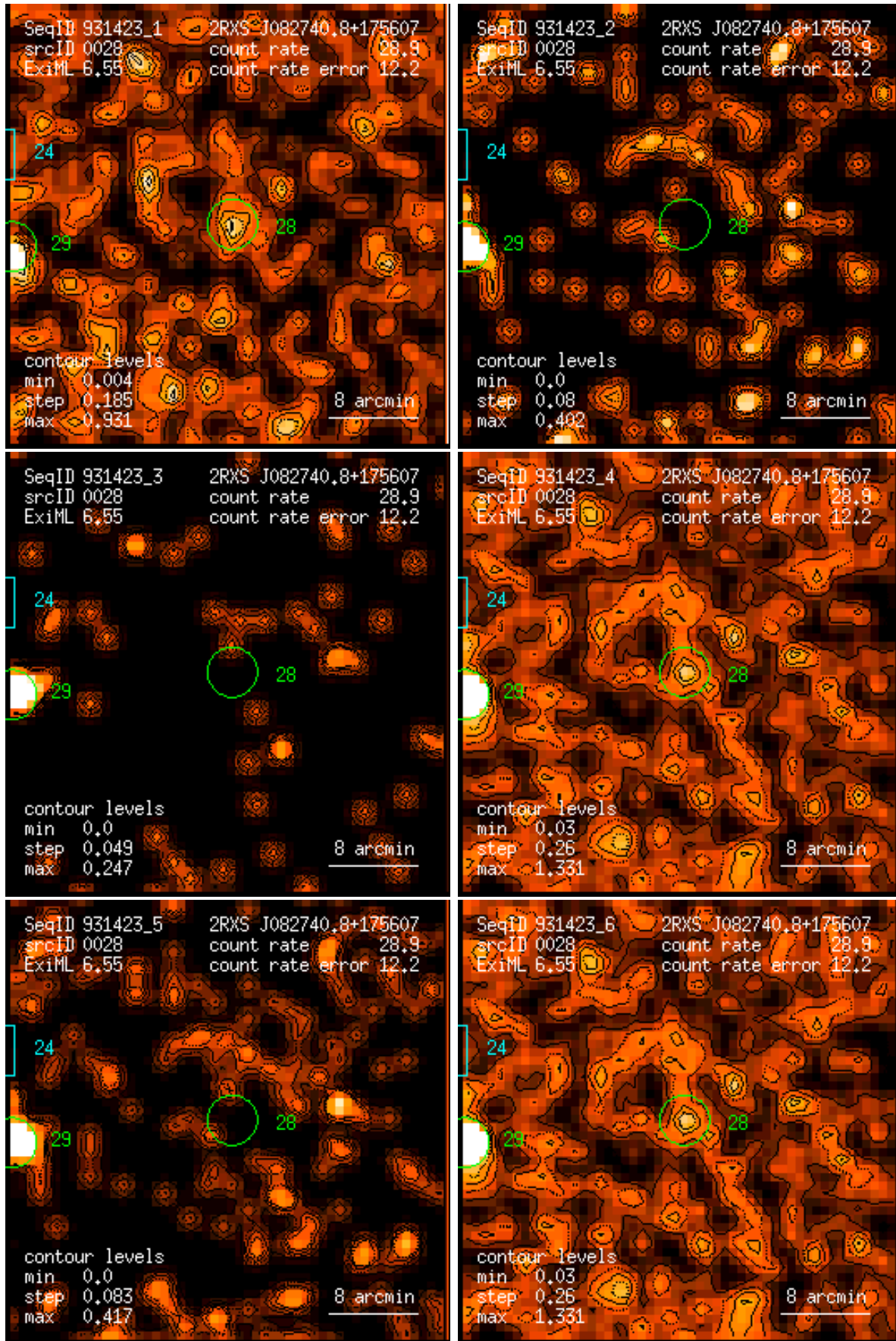
Figure 28: RASS 931423: detection 0028: band rate images, Gaussian filter: (1) PSPC channels 11 – 41, (2) 52 – 90, (3) 91 – 201, (4) 11 – 235, (5) 52 – 201, (6) 11 – 201. Broad band rates in counts/ks. Band rate contour levels in counts/ks/arcmin 2 .
