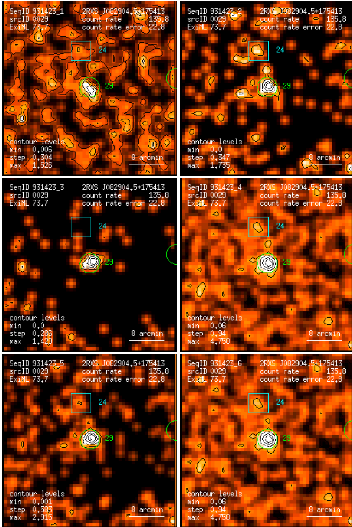
Figure 29: RASS 931423: detection 0029: band rate images, Gaussian filter: (1) PSPC channels 11 – 41, (2) 52 – 90, (3) 91 – 201, (4) 11 – 235, (5) 52 – 201, (6) 11 – 201. Broad band rates in counts/ks. Band rate contour levels in counts/ks/arcmin 2 .
